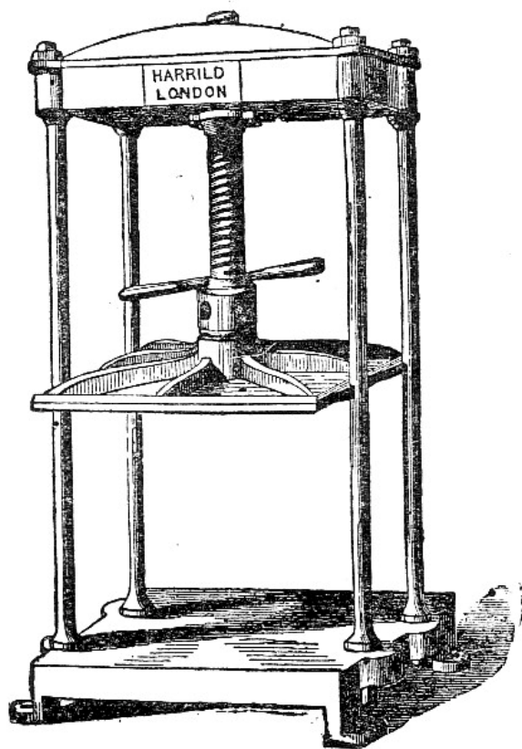
Fig. 2.—Standing Press.
