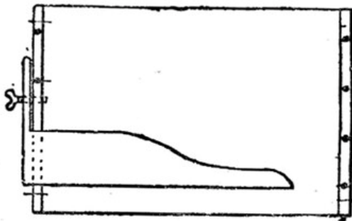
Fig. 26.—Gauge of Strawboard Cutter.
