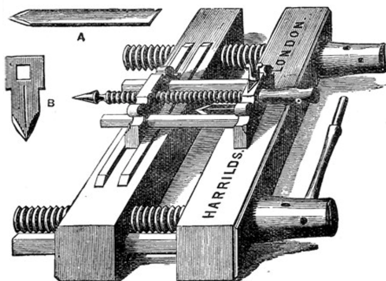
Fig. 12.—Lying Press.
