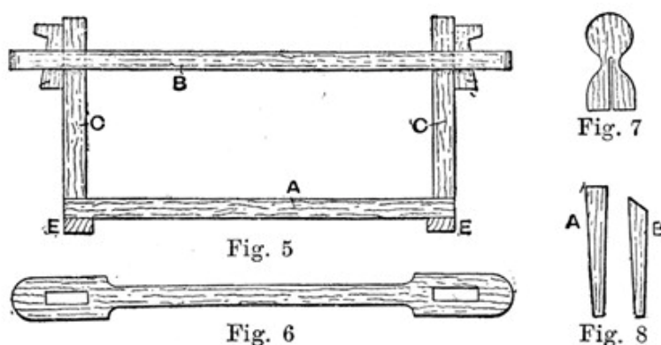
Figs. 5 to 8.—Details of Home-made Sewing Press.
