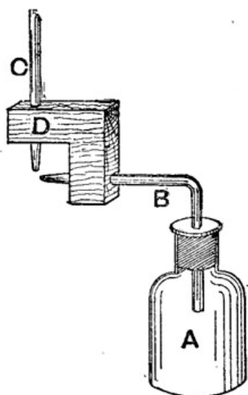
Fig. 48.—Sprayer for Colouring Book Edges.
