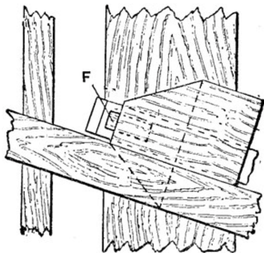
Fig. 20.—Wedges and Chisel of Home-made Plough.
