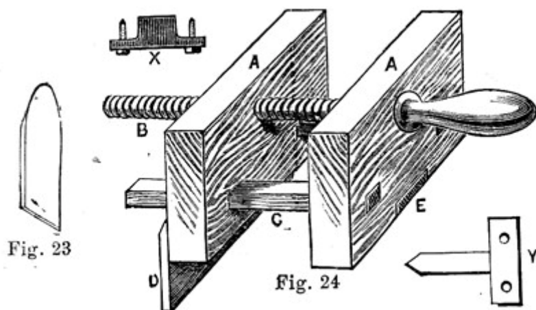
Fig. 23.—Plough Knife. Fig. 24.—Plough.
