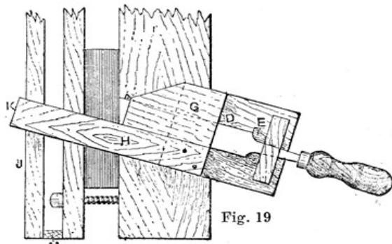
Fig. 18.—Elevation of Home-made Plough. Fig. 19.—Plan of Home-made Plough.
