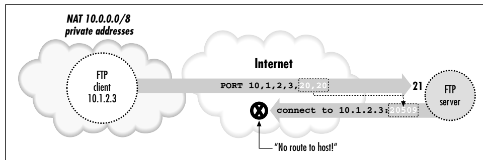
Figure 11-5. Client-side NAT prevents active-mode FTP transfers
