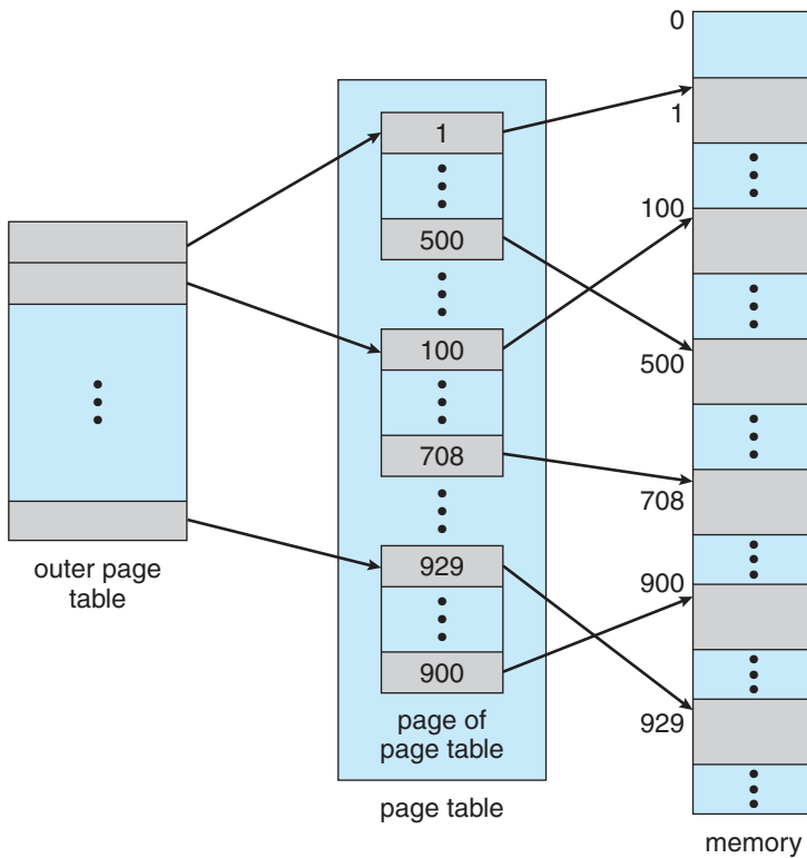
Figure 8.17 A two-level page-table scheme.
