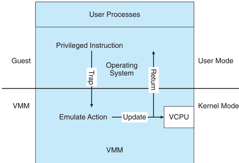
Figure 16.2 Trap-and-emulate virtualization implementation.
