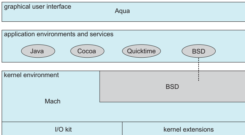
Figure 2.16 The Mac OS X structure.
