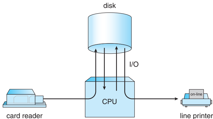
Figure 20.5 Spooling.
