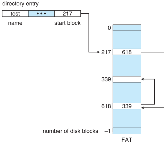
Figure 12.7 File-allocation table.
