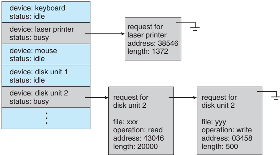
Figure 13.9 Device-status table.
