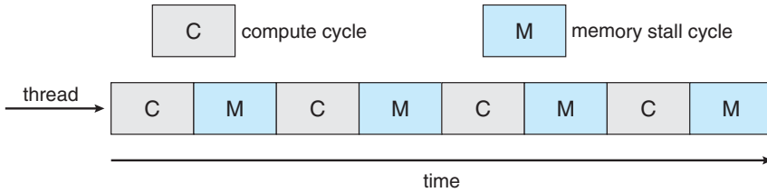
Figure 6.10 Memory stall.
