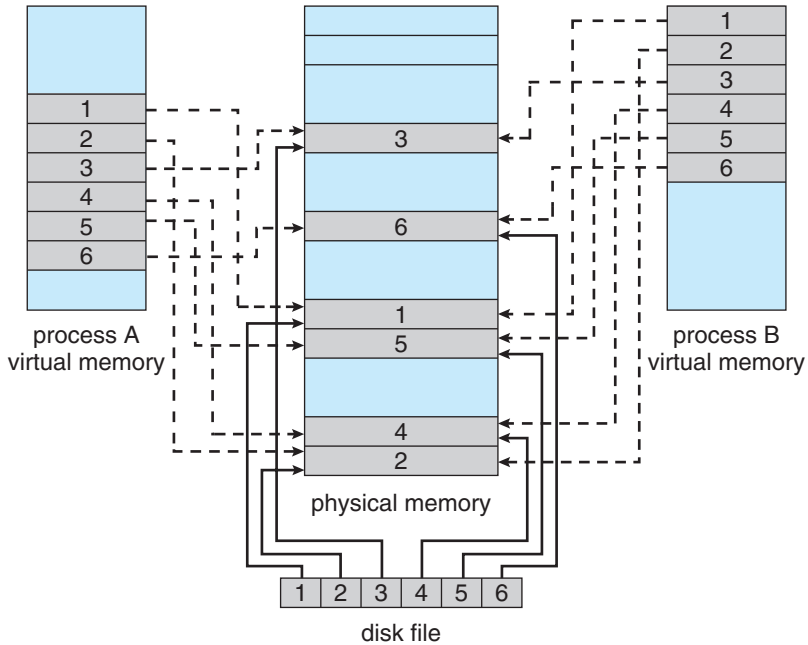
Figure 9.22 Memory-mapped files.
