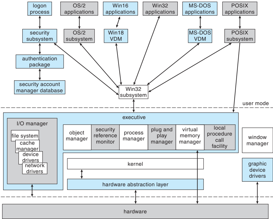
Figure 19.1 Windows block diagram.
