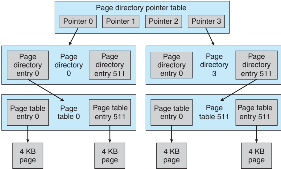
Figure 19.3 Page-table layout.
