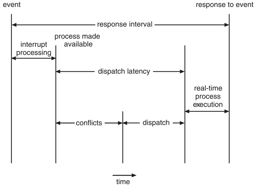
Figure 6.14 Dispatch latency.
