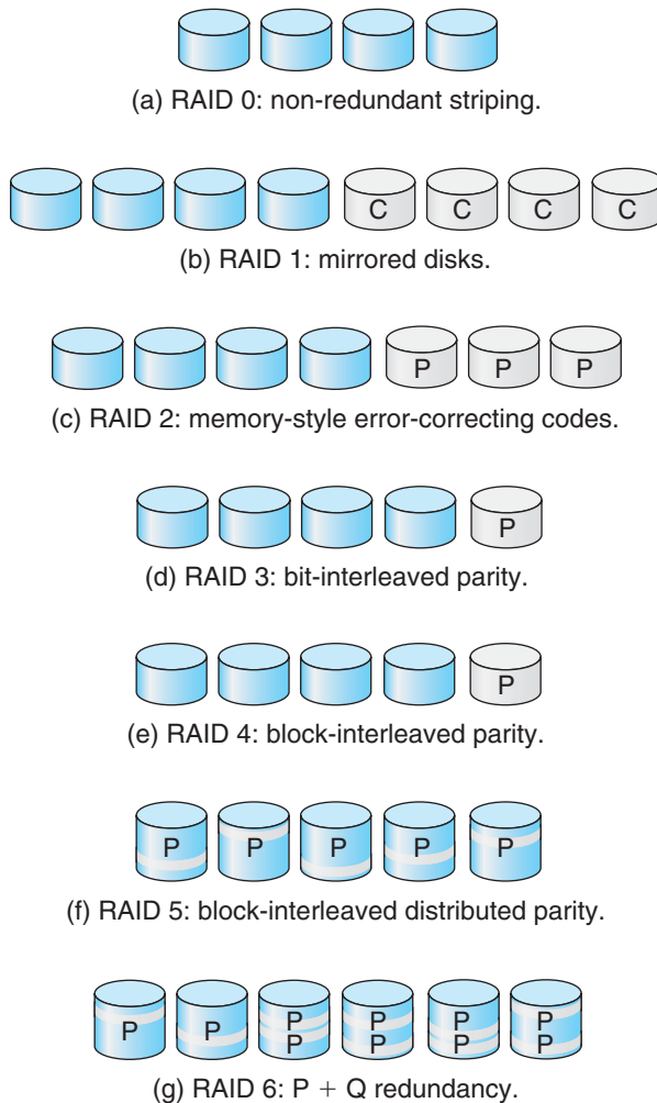
Figure 10.11 RAID levels.
