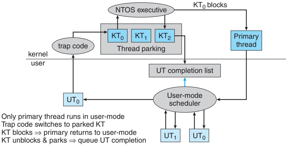
Figure 19.11 User-mode scheduling.
