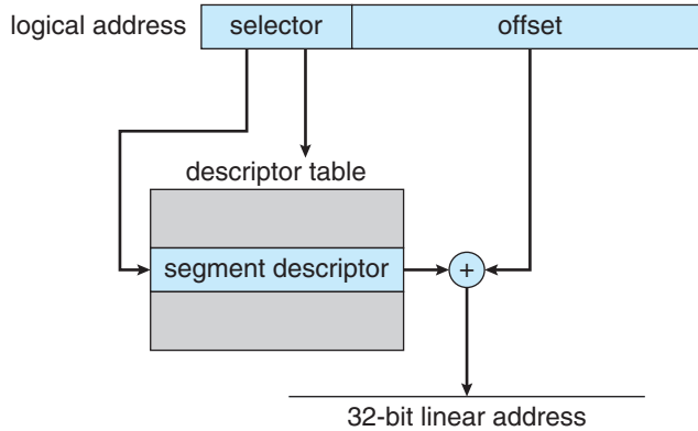
Figure 8.22 IA-32 segmentation.
