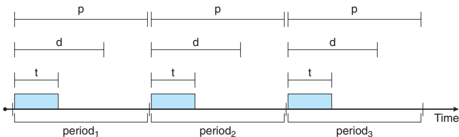
Figure 6.15 Periodic task.
