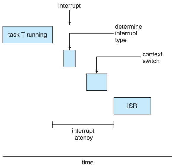
Figure 6.13 Interrupt latency.
