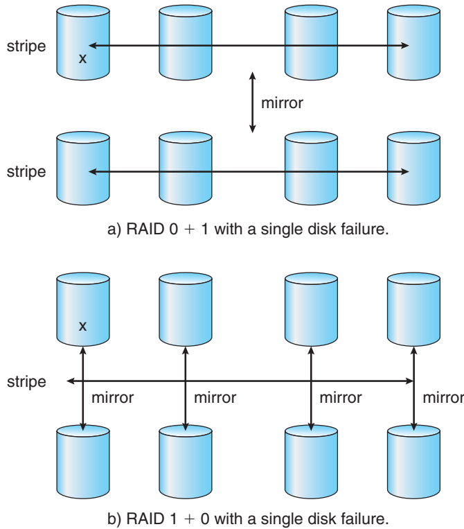
Figure 10.12 RAID 0 + 1 and 1 + 0.
