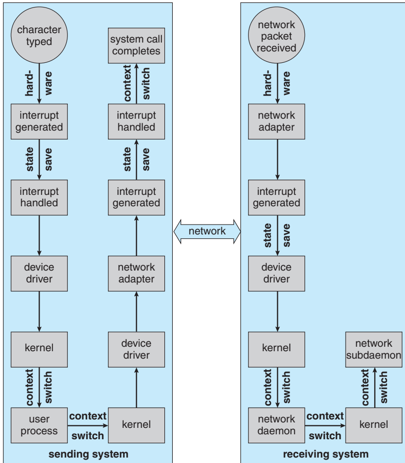
Figure 13.15 Intercomputer communications.
