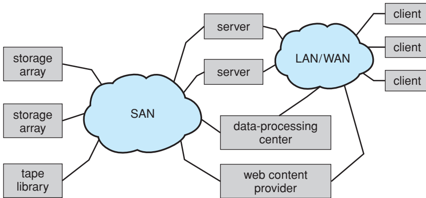
Figure 10.3 Storage-area network.
