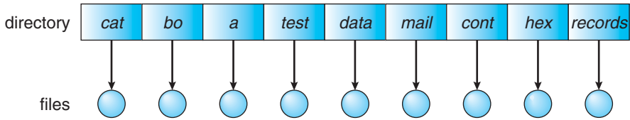
Figure 11.9 Single-level directory.
