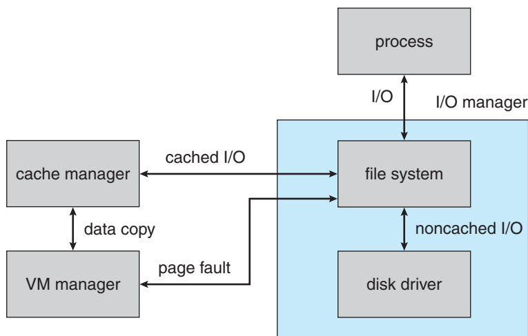
Figure 19.6 File I/O.
