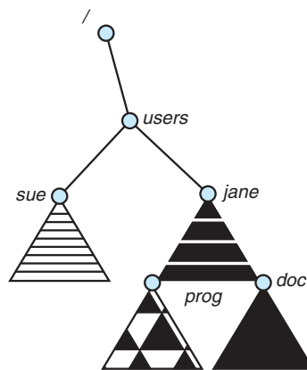
Figure 11.15 Mount point.
