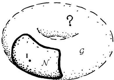
Fig. 13.12 The Lie algebra for a (faithful) representation of a Lie group \mathcal{G} (basically, knowledge of the structure constants \gamma_{\alpha\beta}{}^{\gamma} ) determines the local structure of \mathcal{G} , i.e. it fixes the structure of \mathcal{G} within some (sufficiently small) open region \mathcal{N} surrounding the identity element \mathbf{I} , but it does not tell us about the global nature of \mathcal{G} .
