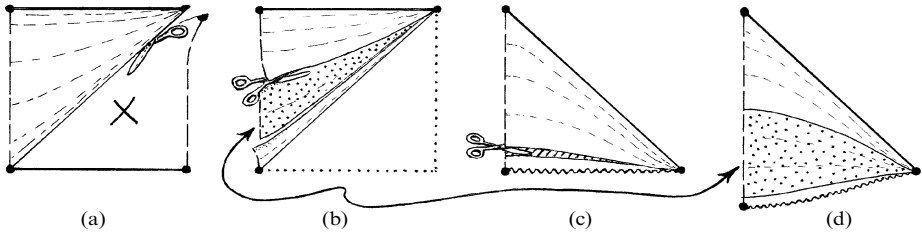
Fig. 28.10 Kit for constructing an inflationary-universe model. (a) de Sitter space cut to give steady-state model. (b) Greatly inflating portion, of steady-state model selected, between two constant-time lines. (c) Small constant-time interval removed from K = 0 FLRW model. (d) Portion from b inserted into c to obtain inflationary universe model. This moves the Big Bang back, as in Fig. 28.5b.
