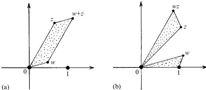
Fig. 5.1 Geometrical description of the basic laws of complex-number algebra. (a) Parallelogram law of addition: 0, w, w + z, z give the vertices of a parallelogram. (b) Similar-triangle law of multiplication: the triangles with vertices 0, 1, w and 0, z, wz are similar.
