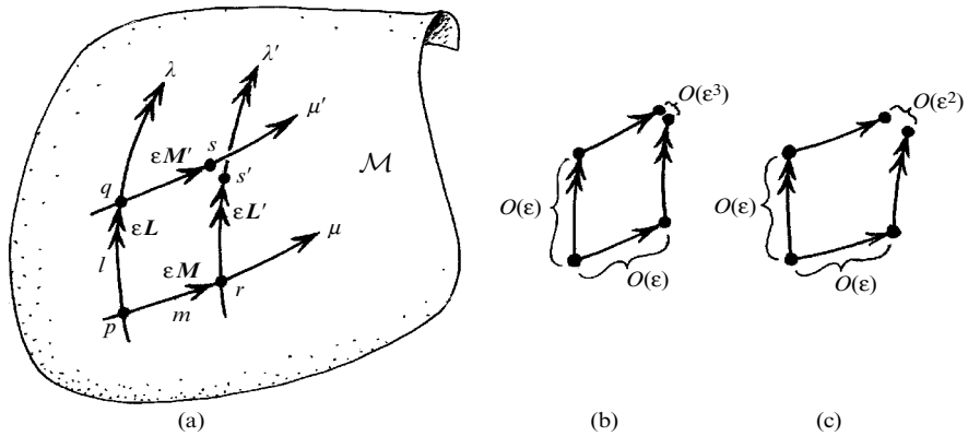
Fig. 14.9 (a) Try to make parallelogram out of geodesics. Take two geodesics \lambda, \mu , through p , in \mathcal{M} , with respective tangent vectors \mathbf{L}, \mathbf{M} at p and corresponding affine parameters l, m . Take q an affine distance l = \epsilon along \lambda from p , and r an affine distance m = \epsilon along \mu from p (with \epsilon > 0 a fixed small number). The geodesic segments pq and pr have respective ‘arrow-lengths’ \epsilon \mathbf{L}, \epsilon \mathbf{M} . To make the parallelogram, move \mathbf{M} from p to q along \lambda by parallel transport ( \nabla_{\mathbf{L}} \mathbf{M} = 0 along \lambda ) giving us a neighbouring geodesic \mu' to \mu , extending from q to s along \mu' by an affine distance \epsilon along the new ‘parallel’ arrow \epsilon \mathbf{M}' . Similarly, move \mathbf{L} from p to r by parallel transport along \mu , and extend from r to s' by a parallel arrow \epsilon \mathbf{L}' measured out from q an affine distance m = \epsilon along \lambda' . (b) Generally s \neq s' and the parallelogram fails to close exactly, but this gap is only O(\epsilon^3) if the torsion \tau vanishes. (c) If there is a non-zero torsion \tau , this will show up as an O(\epsilon^2) term.
