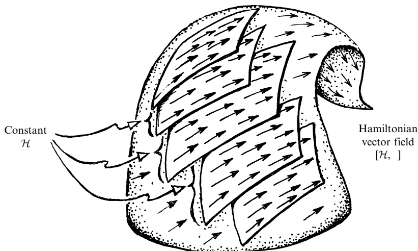
Fig. 20.5 The Hamiltonian flow \{\mathcal{H}, \ \} , representing the Newtonian time-evolution of the system (see §20.4), is a vector field on phase space T^*(C) . For the hypersurfaces of fixed \mathcal{H} -values (fixed energy, taking \mathcal{H} to be time independent), the trajectories remain within the fixed- \mathcal{H} hypersurface, in accordance with energy conservation.
