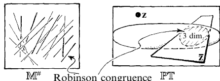
Fig. 33.14 We can obtain a ‘real’ picture of a non-null twistor Z^\alpha by first passing to its complex conjugate \bar{Z}_\alpha , thus defining a complex projective plane in \mathbb{P}^3\mathbb{T} . This plane is fixed by its intersection with \mathbb{P}^3\mathbb{N} , which is a 3-real-dimensional locus. This locus defines a 3-parameter family of light rays in \mathbb{M}^\# called a Robinson congruence.
