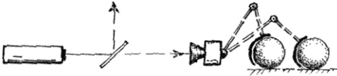
Fig. 30.20 Schrödinger's 'cat' of Fig. 29.7, but now the resulting quantum superposition is merely between two slightly differing locations of a lump of matter.
