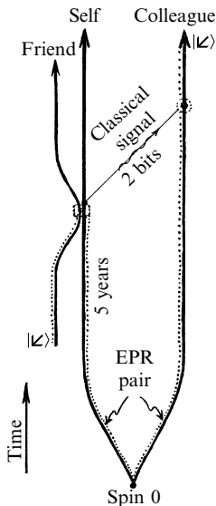
Fig. 23.7 ‘Quantum teleportation’, demonstrating the acausal propagation of quanglement. A space-time diagram illustrates the process whereby the unknown quantum state ( |\mathcal{L}\rangle ) of spin \frac{1}{2} , given to me by my friend, can be conveyed to my colleague on Titan by the mere transmission of 2 bits of classical information, provided that my colleague and I already share an EPR pair. The acausal quanglement link is depicted as a dotted path.
