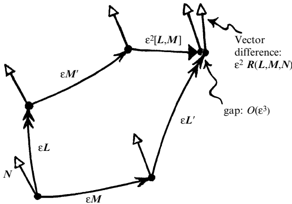
Fig. 14.19 Curvature, in the ‘mathematician’s notation’ (\nabla_L M - \nabla_M L - [L, M])N = R(L, M, N) , from the O(\epsilon^2) discrepancy in parallel transport of a vector N around the (incomplete) ‘quadrilateral’ with sides \epsilon L, \epsilon M, \epsilon L', \epsilon M' . The Lie bracket contribution \epsilon^2[L, M] fills an O(\epsilon^2) gap, to order O(\epsilon^3) . (The index form of the vector R(L, M, N) is L^a M^b N^c R_{abc}{}^d .)
