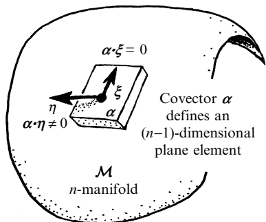
Fig. 12.7 A (non-zero) covector \alpha at a point of \mathcal{M} , determines an (n - 1) -dimensional plane element there. The vectors \xi satisfying \alpha \cdot \xi = 0 define the directions within it.
