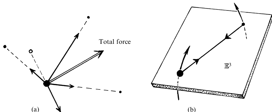
Fig. 17.4 (a) Newtonian force: at any one time, the total force on a particle (double shafted arrow) is the vector sum of contributions (attractive or repulsive) from all other particles. (b) Two particle world lines and the force between them, acting ‘instantaneously’, in a line joining the two particles, at any one moment, within the particular \mathbb{E}^3 that the moment defines. Newton’s Third Law asserts that force on one, as exerted by the other, is equal in magnitude and opposite in direction to the force on the other as exerted by the one.
