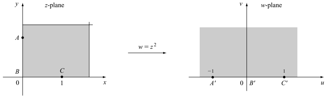
Figure 30.3. The mapping w = z^2 .
