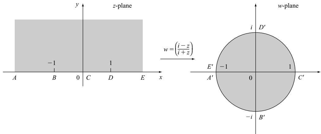
Figure 30.5. The mapping w = \frac{i-z}{i+z} .
