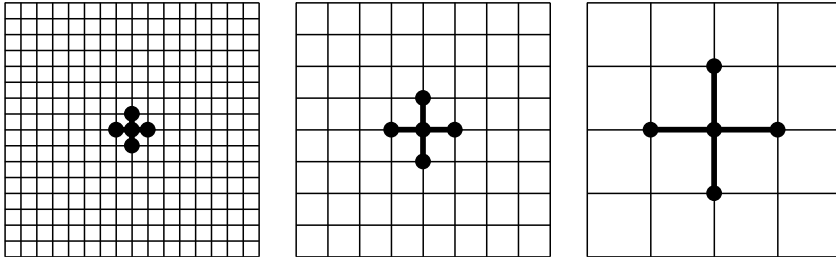
Fig. 12.8. Relation between information exchange and grid size due to neighboring relations of discretization schemes
