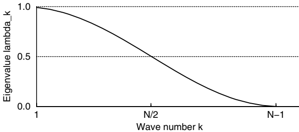
Fig. 12.7. Eigenvalue distribution of iteration matrix of damped Jacobi method for one-dimensional diffusion problem
