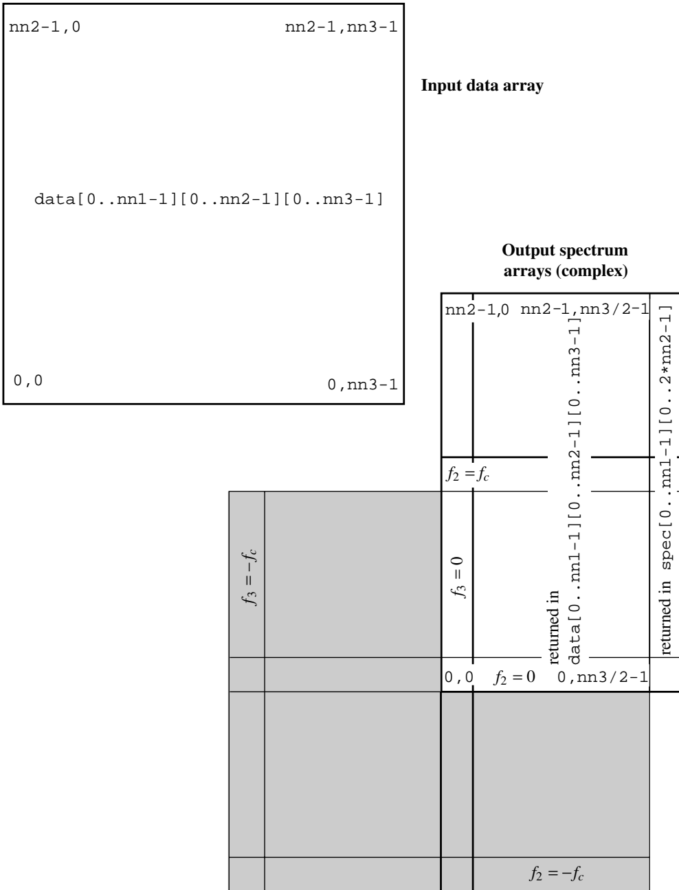
Figure 12.6.1. Input and output data arrangements for rlift3 . All arrays shown are presumed to have a first (leftmost) dimension of range [0..nn1-1] , coming out of the page. The input data array is a real three-dimensional array data[0..nn1-1][0..nn2-1][0..nn3-1] . (For two-dimensional data, one sets nn1 = 1 .) The output data can be viewed as a single complex array with dimensions [0..nn1-1][0..nn2-1][0..nn3/2] (cf. equation 12.6.3), corresponding to the frequency components f_1 and f_2 being stored in wraparound order, but only positive f_3 values being stored (others being obtainable by symmetry). The output data are actually returned mostly in the input array data , but partly stored in the real array spec[0..nn1-1][0..2*nn2-1] . See text for details.
