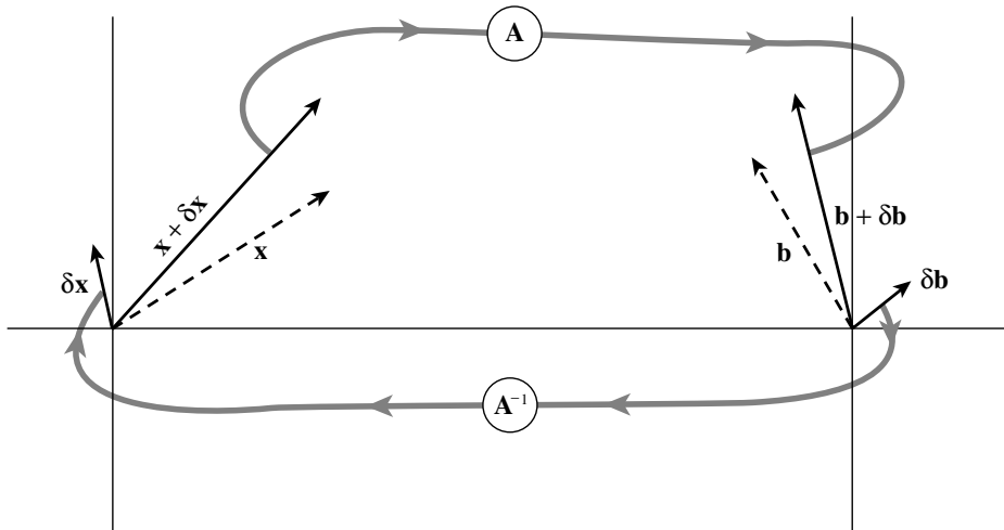
Figure 2.5.1. Iterative improvement of the solution to \mathbf{A} \cdot \mathbf{x} = \mathbf{b} . The first guess \mathbf{x} + \delta \mathbf{x} is multiplied by \mathbf{A} to produce \mathbf{b} + \delta \mathbf{b} . The known vector \mathbf{b} is subtracted, giving \delta \mathbf{b} . The linear set with this right-hand side is inverted, giving \delta \mathbf{x} . This is subtracted from the first guess giving an improved solution \mathbf{x} .
