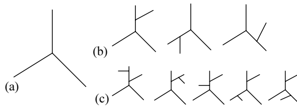
Figure 16.4.3. Tree counting. (a) There is just one unrooted tree with three leaves. (b) There are three ways to add a fourth leaf. (c) For each of the trees in (b), there are five ways to add a fifth leaf. Continuing to add leaves, the number of trees with n leaves is 1 \times 3 \times 5 \times \cdots \times (2n - 5) .
