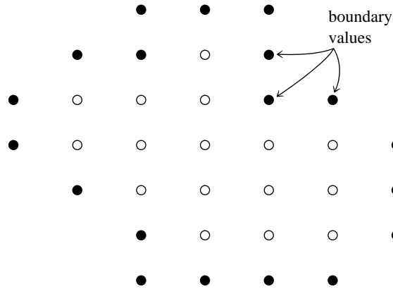
Figure 19.0.1. Initial value problem (a) and boundary value problem (b) are contrasted. In (a) initial values are given on one “time slice,” and it is desired to advance the solution in time, computing successive rows of open dots in the direction shown by the arrows. Boundary conditions at the left and right edges of each row (⊗) must also be supplied, but only one row at a time. Only one, or a few, previous rows need be maintained in memory. In (b), boundary values are specified around the edge of a grid, and an iterative process is employed to find the values of all the internal points (open circles). All grid points must be maintained in memory.
