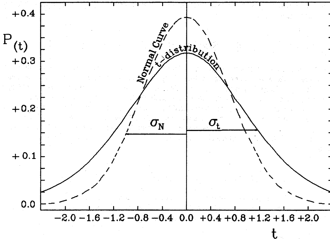
Figure 8.1 shows a comparison between the normal curve and the t -distribution function for N=8 . The symmetric nature of the t -distribution means that the mean, median, mode, and skewness will all be zero while the variance and kurtosis will be slightly larger than their normal counterparts. As N \rightarrow \infty , the t -distribution approaches the normal curve with unit variance.
