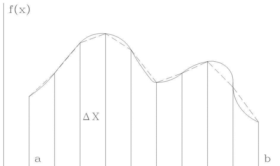
Figure 4.1 shows a function whose integral from a to b is being evaluated by the trapezoid rule. In each interval a straight line approximates the function \Delta x_i .
