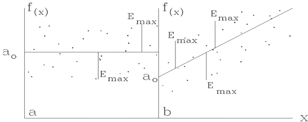
Figure 6.4 shows the Chebyshev fit to a finite set of data points. In panel a the fit is with a constant a_0 while in panel b the fit is with a straight line of the form f(x) = a_1x + a_0 . In both cases, the adjustment of the parameters of the function can only produce (n+2) maximum errors for the (n+1) free parameters.
