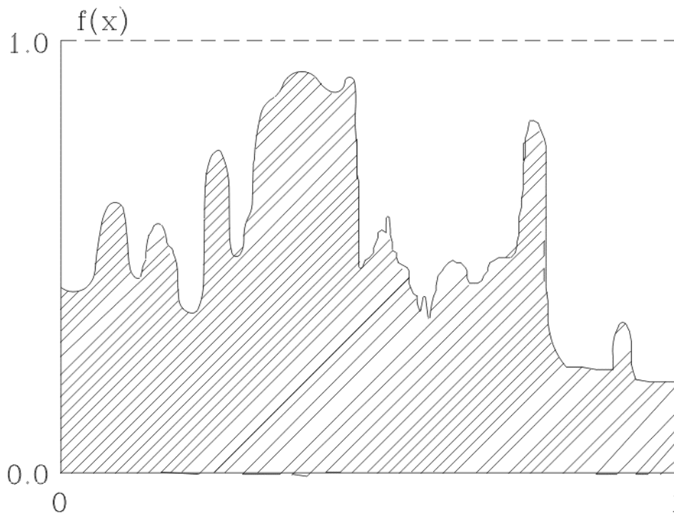
Figure 4.2 shows the variation of a particularly complicated integrand. Clearly it is not a polynomial and so could not be evaluated easily using standard quadrature formulae. However, we may use Monte Carlo methods to determine the ratio area under the curve compared to the area of the rectangle.
