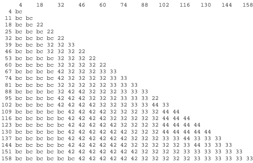
Figure 1.1 The best algorithm to multiply two numbers of x and y words for 4 \leq x \leq y \leq 158 : bc is schoolbook multiplication, 22 is Karatsuba's algorithm, 33 is Toom-3, 32 is Toom-(3, 2), 44 is Toom-4, and 42 is Toom-(4, 2). This graph was obtained on a Core 2, with GMP 5.0.0, and GCC 4.4.2. Note that for x \leq (y + 3)/4 , only the schoolbook multiplication is available; since we did not consider the algorithm that cuts the larger operand into several pieces, this explains why bc is best for say x = 32 and y = 158 .
