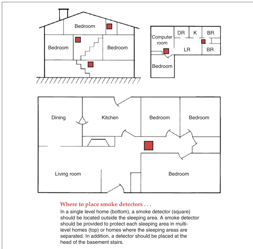
A simple drawing showing where to place smoke detectors in a house. Figure 10.23
