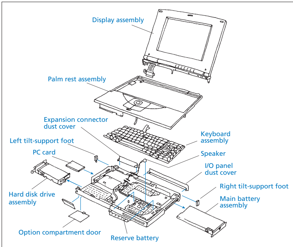
Exploded drawing of a notebook.
