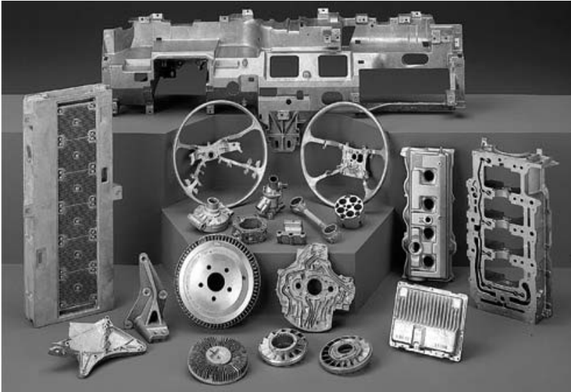
Figure 3.11 Components manufactured using vacuum die casting. (Courtesy of Gibbs Die Casting Corporation.)
