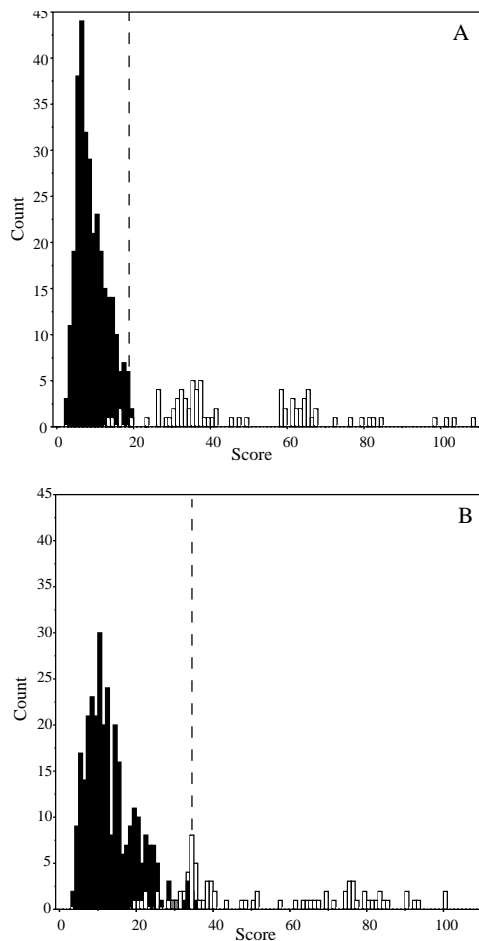
Figure 14. Match score distributions comparing AACC pattern vs. sequence matches (A) to sequence vs. sequence matches (B). (A) An AACC pattern was constructed from 4 protein tyrosine kinase sequences (Fig. 14C) and matched to 2 control sets: a positive control set composed of 81 protein kinase (PK) related sequences (white bars) and a negative control set 313 non-PK-related sequences (black bars; \text{mean} \pm \text{s.d.} = 10.88 \pm 4.60 ); where the two sets of matches overlap, the smaller bar at each position is shown in the foreground; at those positions where the bars are the same height, a single stippled bar is displayed. The dashed line indicates the 99th percentile of the negative control scores. (B) Score distributions of a single PK sequence (human ret , locus TVHURE ) matched against the same positive (white bars) and negative (black bars; \text{mean} \pm \text{s.d.} = 13.59 \pm 6.59 ) control sets described above. As in (A), the dashed line indicates the 99th percentile of the negative control set. [From Smith and Smith, 1990]
