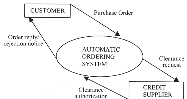
Figure 8 A context diagram.
