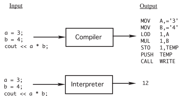
Figure 1 A compiler and interpreter producing very different output for the same input.
