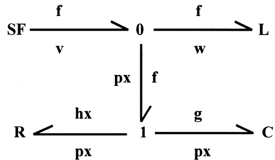
Figure 17 Bond graph model for the system of Fig. 17.
