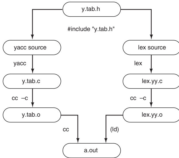
Figure 18 Generation and compilation of software using lex and yacc.
