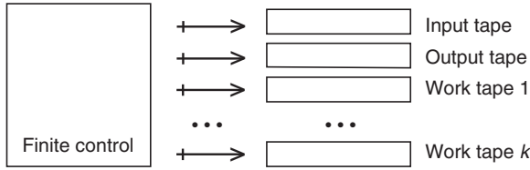
Figure 1 Schematic of a finite state machine. The \leftrightarrow symbol denotes sequential access to a tape.
