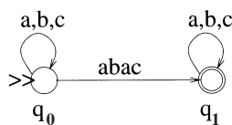
Figure 8 An NFA for accepting the language \{x \mid x \in \{a, b, c\}^* \text{ and } x \text{ contains the pattern } abac\} .
