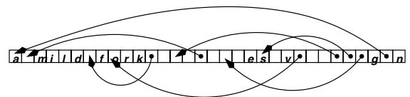
Figure 8 Illustration for LZ77.
