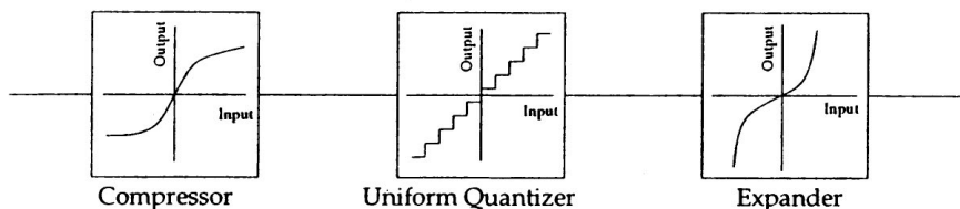
Figure 10 Companded quantization.
