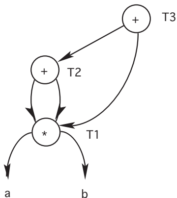
Figure 28 Example of a DAG.
