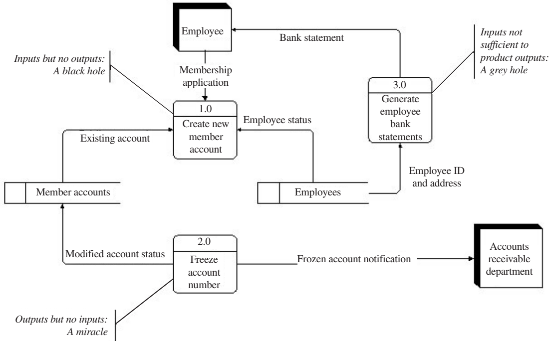
Figure 5 Common DFD drafting errors: black holes, gray holes, miracles. [Adapted from Figure 9.5, p. 356 in Whitten, J. L., Bentley, L. D., and Barlow, V. M. (1994). Systems Analysis and Design Methods (3rd Ed.). Burr Ridge, IL: Irwin.]
