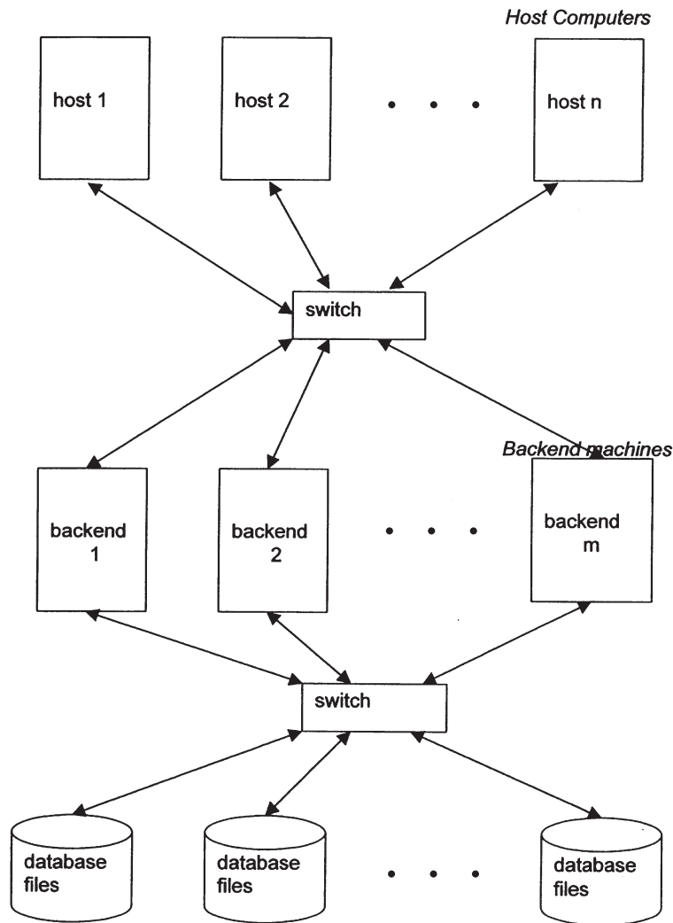
Figure 2 Parallel architecture.
