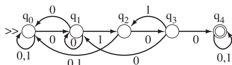
Figure 13 A sample NFA.
