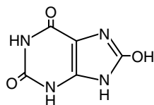
Uric acid
