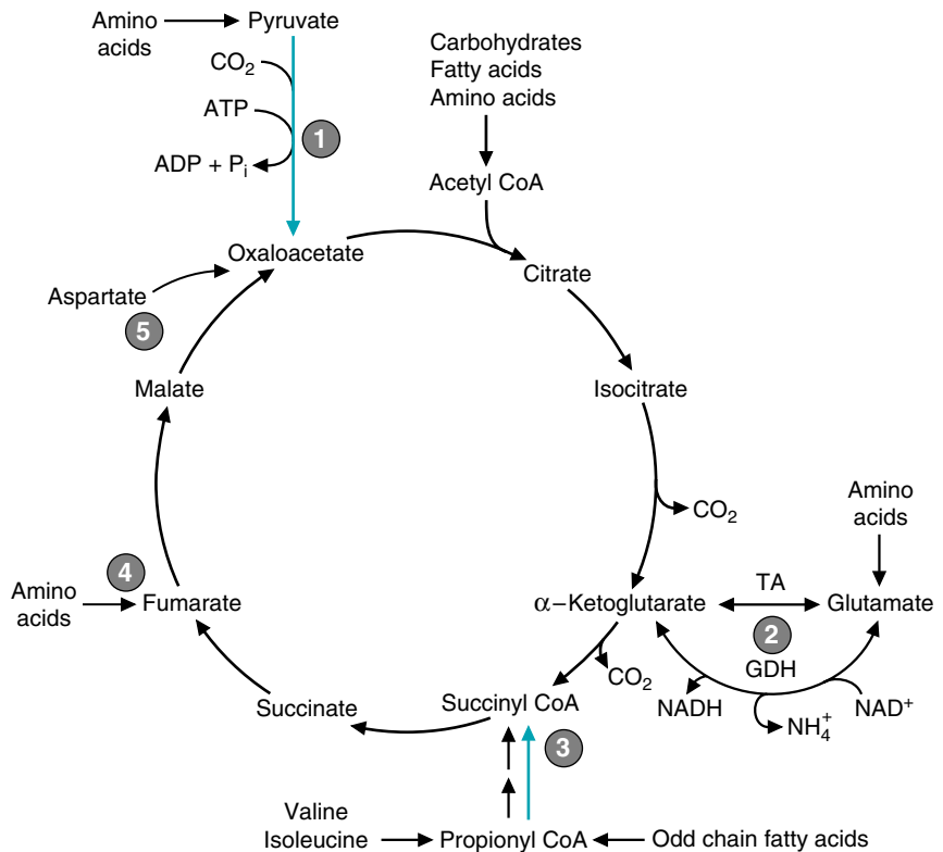
Fig. 20.19. Major anaplerotic pathways of the TCA cycle. 1 and 3 (blue arrows) are the two major anaplerotic pathways. (1) Pyruvate carboxylase (2) Glutamate is reversibly converted to \alpha -ketoglutarate by transaminases (TA) and glutamate dehydrogenase (GDH) in many tissues. (3) The carbon skeletons of valine and isoleucine, a 3-carbon unit from odd chain fatty acid oxidation, and a number of other compounds enter the TCA cycle at the level of succinyl CoA. Other amino acids are also degraded to fumarate (4) and oxaloacetate (5), principally in the liver.
