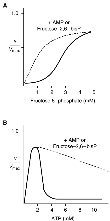
Fig. 22.14. Regulation of PFK-1 by AMP, ATP and fructose-2,6-bisP. A. AMP and fructose 2,6-bisphosphate activate PFK-1. B. ATP increases the rate of the reaction at low concentrations, but allosterically inhibits the enzyme at high concentrations.
