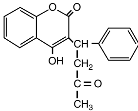
Warfarin
