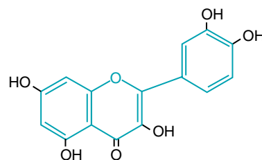
A flavonoid
