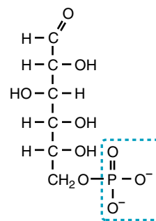
Glucose 6-phosphate
