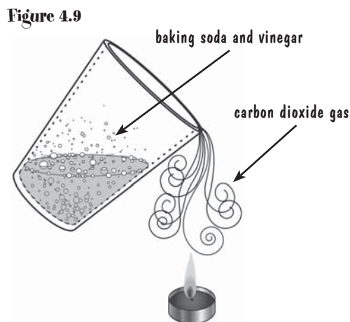
Figure 4.9 "Pouring" carbon dioxide gas over a candle.
