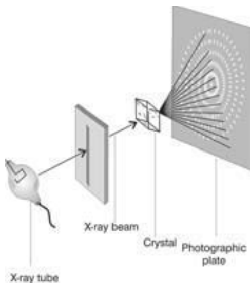
Figure 8.8 Picture of X-ray Diffraction Pattern (Rae Déjur)
