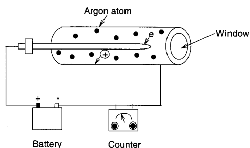
Figure 17.11 A Geiger Counter detects radiation by ionizing argon atoms. The flow of argon ions and electrons in the tube creates a current that is amplified and detected by the counter.
