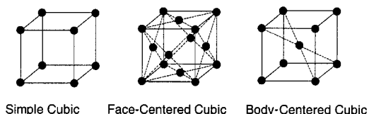
Figure 8.9 Three Simple Unit Cells for Crystalline Solids
