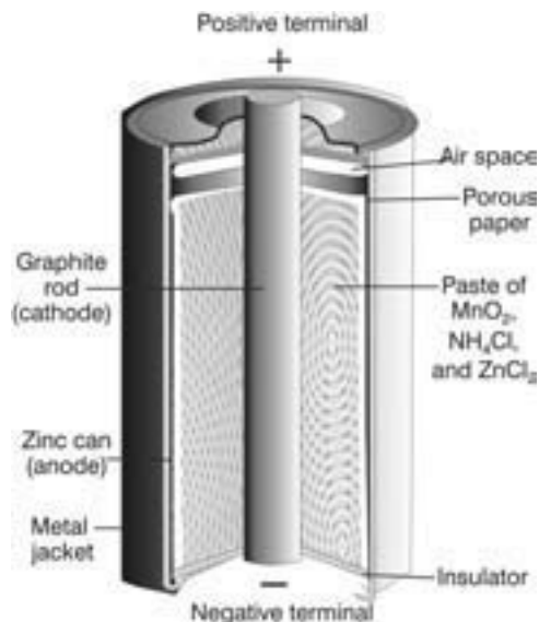
Figure 14.8 Dry Cell Battery (Rae Déjur)
