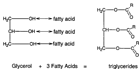
Figure 15.15 A triglyceride forms when three fatty acids react with glycerol. When a triglyceride forms, three molecules of water are produced as a byproduct.
