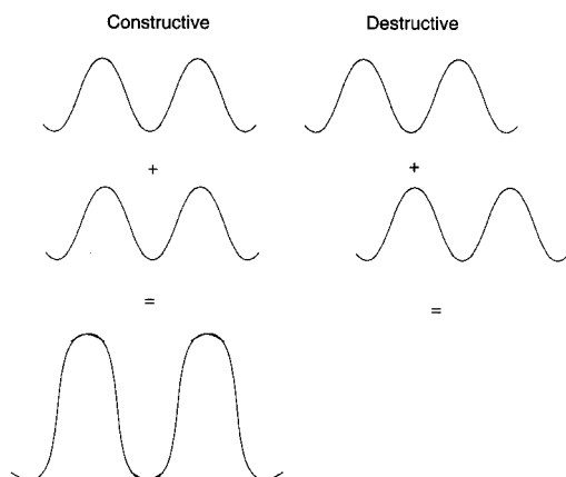
Figure 8.7 In constructive interference, waves reinforce each other. In destructive interference, waves cancel each other.
