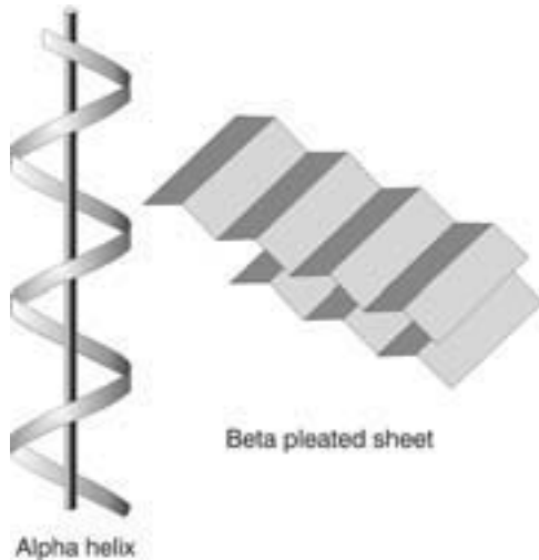
Figure 16.13 The alpha helix and beta sheets are two types of secondary structures exhibited by polypeptides and proteins. (Rae Déjur)
