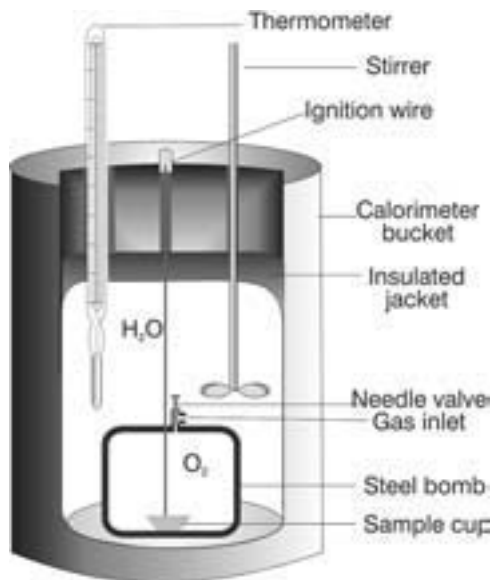
Figure 10.4 Bomb Calorimeter (Rae Déjur)
