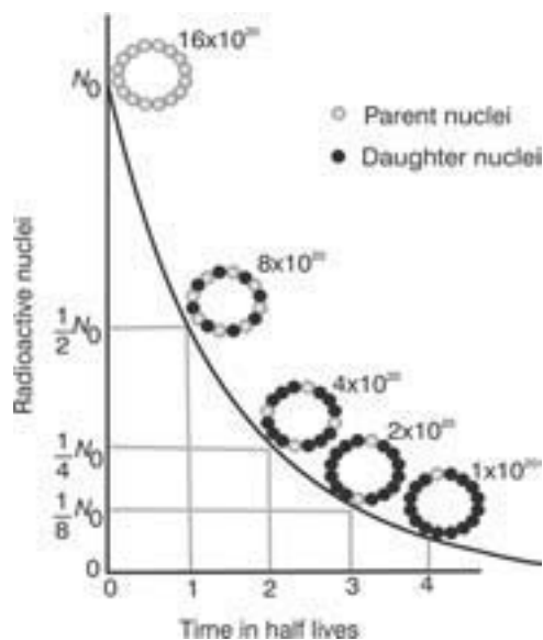
Figure 17.3 Exponential Decay (Rae Déjur)
