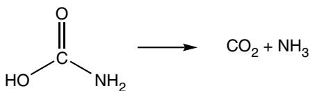
Figure 12-42: The decomposition of carbamic acid.
