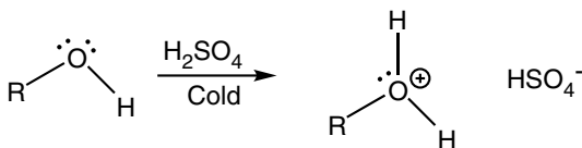
Figure 3-5: Protonation of an alcohol by sulfuric acid.
