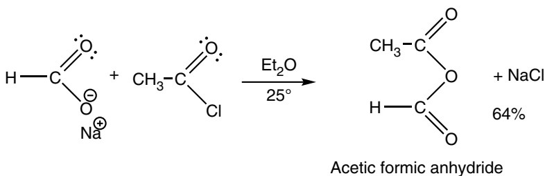
Figure 12-16: The reaction of sodium salt of sodium carboxylic acid (sodium formate) with acid chloride.
