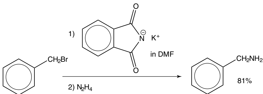
Figure 13-14: Using the Gabriel synthesis to produce an amine.
