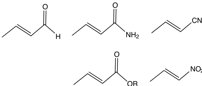
Figure 11-27: Some Michael acceptors.
