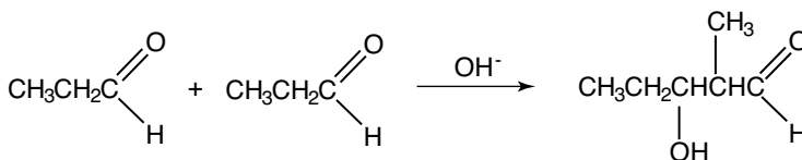
Figure 11-11: An example of an aldol reaction.
