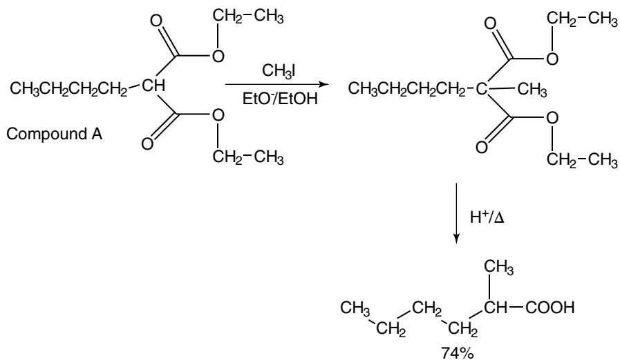
Figure 15-19: Another example of the use of compound A in synthesis.
