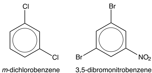
Figure 6-10: Two examples demonstrating different ways of naming aromatic compounds.
