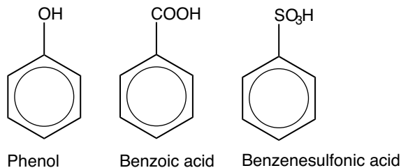
Figure 6-11: Some common names adopted by the IUPAC system through common usage.
