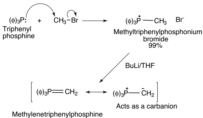
Figure 10-29: The formation of a phosphorus ylide.
