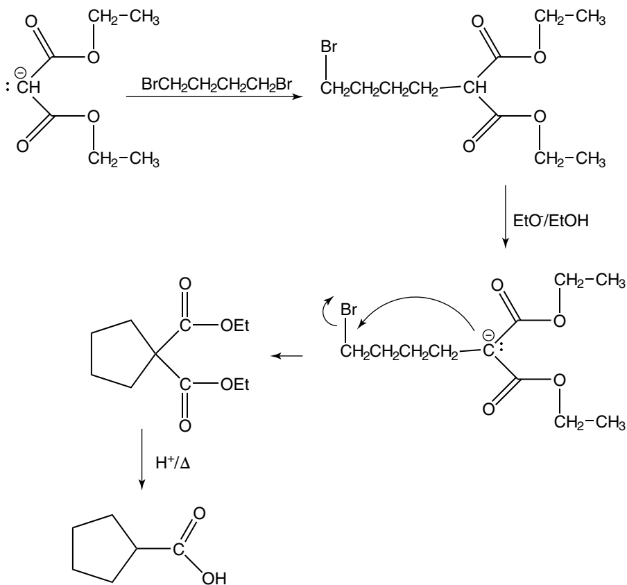
Figure 15-20: Another reaction beginning with the anion in Figure 15-17.
