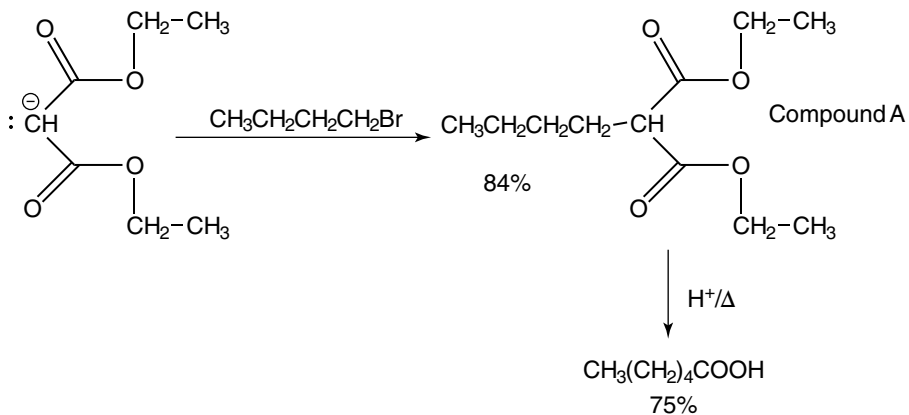
Figure 15-18: Formation of compound A from the anion in Figure 15-17.
