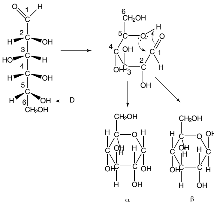
Figure 16-2: Mutarotation in glucose.
