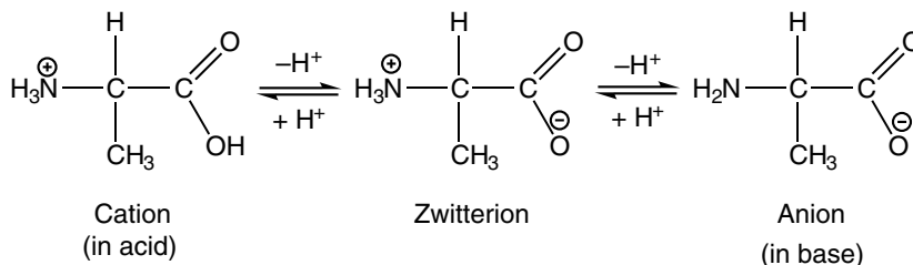
Figure 16-35: The action of an acid and a base upon the zwitterion of alanine ( \text{R} = -\text{CH}_3 ).
