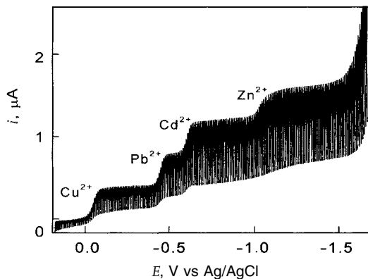
Fig. 5.11 An example of a DC polarogram for a multi-component system. Electroactive species: \text{Cu}^{2+} , \text{Pb}^{2+} , \text{Cd}^{2+} and \text{Zn}^{2+} in 1.0 mM each. Supporting electrolyte: 0.1 M tartaric acid + 0.5 M ammonium acetate.
