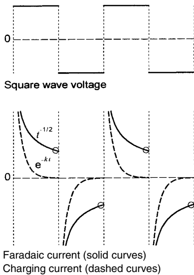
Fig. 5.15 Square-wave voltage (e.g. 200 Hz, 10 mV) (upper) and the faradaic current (solid curve) and the charging current (dashed curve) (lower) in SW polarography. The currents after attenuation of the charging current (shown by small circles) are sampled.
