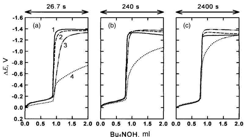
Fig. 6.5 Titration curves of 5 mM picric acid in AN with 1 M \text{Bu}_4\text{NON} (in MeOH), recorded simultaneously with four pH sensors, but at different titration speeds for (a) to (c). In (a), curve 1 is for \text{Si}_3\text{N}_4 -ISFET, 2 for \text{Ta}_2\text{O}_5 -ISFET, 3 for \text{IrO}_2 pH-sensor, and 4 for glass electrode. The pH-ISFETs were obtained from Shindengen Indus. Co. and the \text{IrO}_2 pH-sensor from TOA Electronics Ltd [17c].
