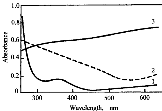
Fig. 5.26 UV/vis absorption curves for OTEs coated on the quartz plate. 1: \text{SnO}_2 ( 20 \Omega \text{ cm}^{-2} ), 2: \text{Au-PbO}_2 ( 11 \Omega \text{ cm}^{-2} ), 3: \text{Pt} ( 20 \Omega \text{ cm}^{-2} ).
