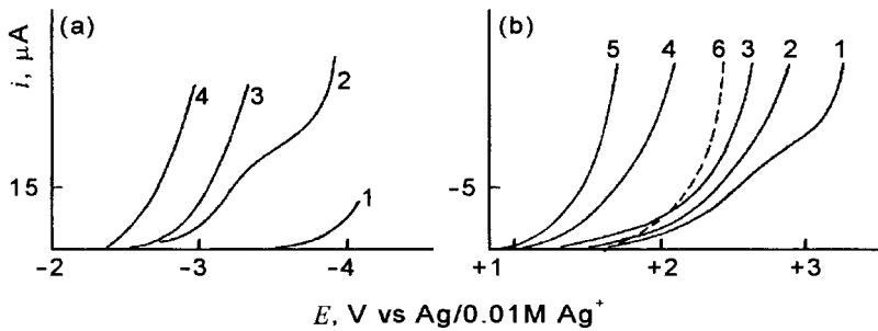
Fig. 10.1 Effect of water on the residual current-potential curves at a platinum electrode in PC [10]. (a) Cathodic side in 0.1 M \text{Bu}_4\text{NClO}_4 . Water concentration: curve 1, \sim 0 M, 2, 0.01 M, 3, 0.03 M, 4, 0.1 M; (b) anodic side in 0.1 M \text{KPF}_6 . Water concentration: curve 1, 0.01 M, 2, 0.03 M, 3, 0.1 M, 4, 0.5 M, 5, 1 M (curve 6 is in 0.1 M \text{LiClO}_4 at a water concentration of 0.001 M).
