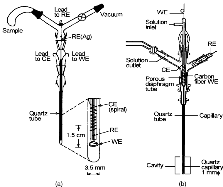
Fig. 9.6 Electrochemical-ESR cells. (a) In situ generation type (Fernando, K.R. et al. J. Mag. Reson. 1986, 68, 552). (b) Ex situ generation type [14].
