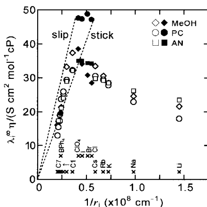
Fig. 7.5 \lambda_i^\infty \eta - r_i^{-1} relation for cations (open symbols) and anions (solid symbols) in MeOH, PC and AN. C1 → C7 means, from right to left, \text{Me}_4\text{N}^+ , \text{Et}_4\text{N}^+ , \text{Pr}_4\text{N}^+ , \text{Bu}_4\text{N}^+ , \text{Am}_4\text{N}^+ , \text{Hex}_4\text{N}^+ and \text{Hep}_4\text{N}^+ . The dashed lines show the theoretical slopes for stick and slip conditions. The data for crystallographic ionic radii (or analogous) and ionic molar conductivities are from Tables 3 and 28 in Marcus, Y. Ion Properties , Marcel Dekker, New York, 1997.
