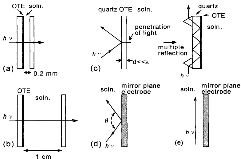
Fig. 9.2 Various methods of spectroelectrochemistry. (a) Transmission method (thin-layer cell), (b) transmission method (cell of conventional thickness), (c) internal reflec-
