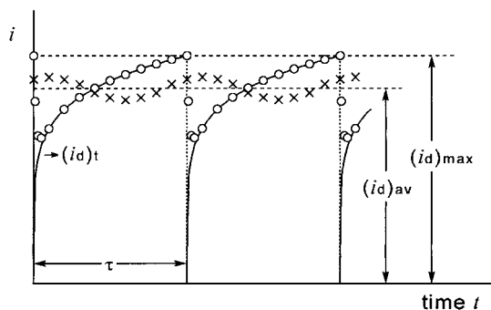
Fig. 5.12 Current-time curve at a DME (solid curve) and the oscillation of the pen recorder measured without (O) and with (X) damping.
