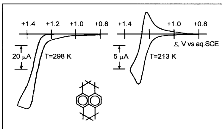
Fig. 8.22 Effect of temperature on the cyclic voltammogram for the oxidation of 1,2,3,6,7,8-hexahydrodipyrene (2.5 mM) at a platinum electrode in 0.1 M Bu 4 NClO 4 -butyronitrile. Scan rate: 50 mV s -1 [76 a]
