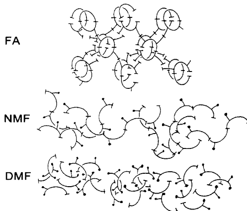
Fig. 1.3 The liquid structures of FA, NMF, and DMF [23]. ● — Methyl group; ⋯ — H-bond (-NH...O=CH-).
