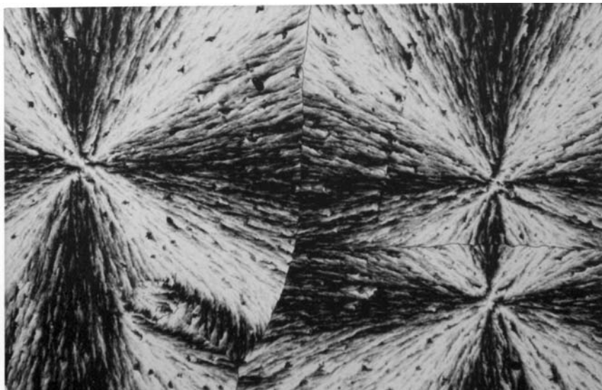
Figure 5.7. Optical microscope image of a thin film (thickness \sim 2 \mu\text{m} ) of \alpha - p -NPNN grown on a glass substrate ( 1.6 \times 1.0 \text{ mm}^2 , crossed polarizers). Reprinted from Journal of Crystal Growth , Vol. 209, J. Caro, J. Fraxedas and A. Figueras, Thickness-dependent spherulitic growth observed in thin films of the molecular organic radical p-nitrophenyl nitronyl nitroxide , 146–158, Copyright (2000), with permission from Elsevier.
