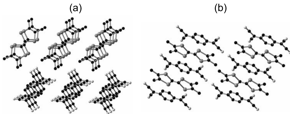
Figure 1.16. Crystal structures of TMTSF-TCNQ. (a) Black phase, P\bar{1} , a = 0.388 nm, b = 0.764 nm, c = 1.885 nm, \alpha = 77.34^\circ , \beta = 89.67^\circ , \gamma = 94.63^\circ . Crystallographic data from Bechgaard et al. , 1977. (b) Red phase, P\bar{1} , a = 0.810 nm, b = 1.046 nm, c = 0.700 nm, \alpha = 103.78^\circ , \beta = 98.49^\circ , \gamma = 94.91^\circ . Crystallographic data from Kistenmacher et al. , 1982. C, S and N are represented by black, medium grey and light grey balls, respectively. H atoms are not represented for clarity.
