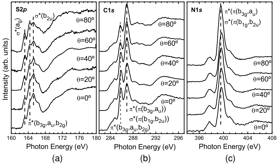
Figure 6.16. Angular dependent NEXAFS spectra of TTF-TCNQ for (a) S2p, (b) C1s and (c) N1s. The \theta_E angle is defined as the angle between the light polarization vector and the surface plane. Reprinted with permission from J. Fraxedas, Y. J. Lee, I. Jiménez, R. Gago, R. M. Nieminen, P. Ordejón and E. Canadell, Physical Review B , 68 , 195115 (2003). Copyright (2003) by the American Physical Society.
