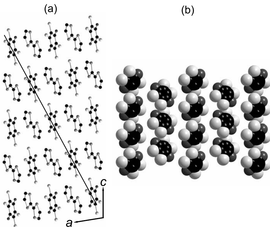
Figure 4.34. Crystal structure of the neutral phase of TTF-CA. Crystallographic data from Le Cointe et al. , 1995. (a) Projection of the ac -plane with the b -direction pointing perpendicular to the plane. The molecular (101) plane, which contains the b -direction, is indicated by a straight line. (b) Space-filling model of the CA (101) plane. C, O, S and Cl are represented by black, dark grey, medium grey and light grey balls, respectively. H atoms are omitted.
