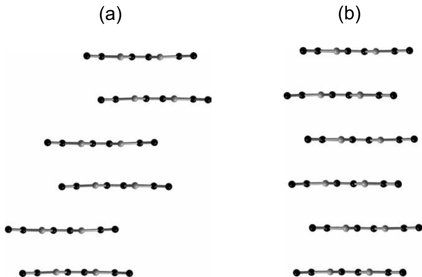
Figure 6.28. Stack of molecules in (a) \mu' -(TMTTF) 2 ReO 4 and (b) in triclinic (TMTTF) 2 ReO 4 . C and S atoms are represented by black and medium grey balls, respectively. H atoms are omitted for clarity.
