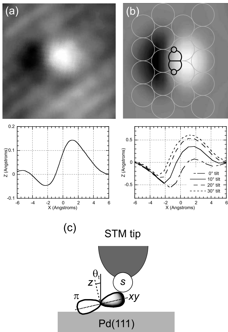
Figure 4.5. (a) 1.2 \text{ nm} \times 1.3 \text{ nm} image of a single C_2H_2 molecule ( V_t = 40 \text{ mV} , I_t = 400 \text{ pA} ). The graph below shows a cross section along a path through the maximum and minimum of the image. (b) 1.2 \text{ nm} \times 1.3 \text{ nm} ESQC calculated STM image for the minimum energy geometry. The calculated image is overlaid on a schematic of the adsorbed molecule. The graph shows the calculated molecular profile vs. molecular tilt angle \theta_t . As \theta_t increases, the protrusion increases as the depression decreases. Reprinted with permission from J. C. Dunphy, M. Rose, S. Behler, D. F. Ogletree, M. Salmeron and P. Sautet, Physical Review B , 57 , R12705 (1998). Copyright (1998) by the American Physical Society. (c) Schematic representation of the orbital interaction of the STM tip/ C_2H_2 /Pd(111) system.
