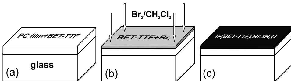
Figure 3.21. Scheme of the preparation by MRDT of a conducting surface layer of \theta -(BET-TTF) 2 Br·3H 2 O nanocrystals on a polycarbonate (PC) substrate. Adapted from Mas-Torrent et al. , 2001.
