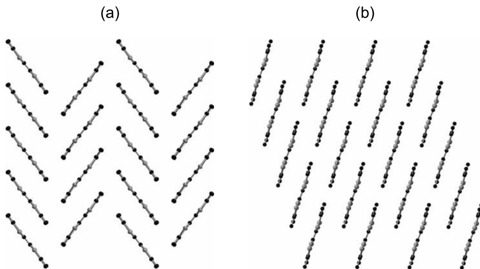
Figure 1.10. (a) (\bar{2}02) plane of TMTTF and (b) (100) plane of TMTSF. TMTTF: C2/c , a = 1.614 nm, b = 0.606 nm, c = 1.428 nm, \beta = 119.974^\circ . TMTSF: P\bar{1} , a = 0.693 nm, b = 0.809 nm, c = 0.631 nm, \alpha = 105.51^\circ , \beta = 95.39^\circ , \gamma = 108.90^\circ . Crystallographic data from Kistenmacher et al. , 1979.
