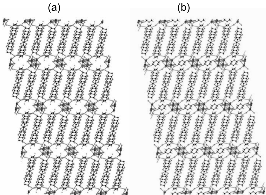
Figure 6.26. Projected view along the a -direction of (a) \beta'' -(BEDT-TTF) _4 ·(H _2 O) _2 ·[Re _6 S _6 Cl _8 ], P\bar{1} , a = 0.910 nm, b = 2.006 nm, c = 1.157 nm, \alpha = 84.380^\circ , \beta = 101.405^\circ , \gamma = 79.318^\circ and (b) \beta'' -(BEDT-TTF) _4 ·(C _4 H _8 O _2 )·[Re _6 S _6 Cl _8 ], P\bar{1} , a = 0.910 nm, b = 2.003 nm, c = 1.170 nm, \alpha = 84.85^\circ , \beta = 101.32^\circ , \gamma = 78.495^\circ . Crystallographic data from Deluzet et al. , 2002a.
