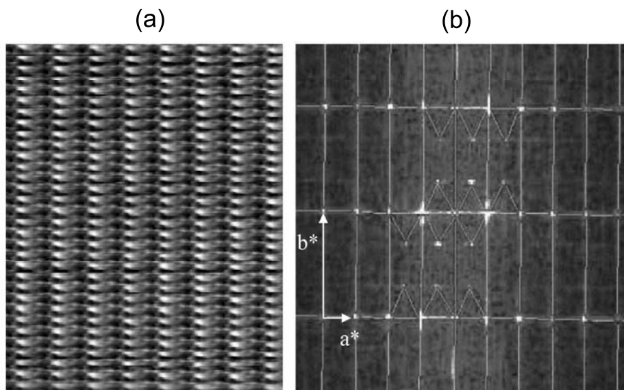
Figure 6.19. (a) STM image of the ab -plane of TTF-TCNQ taken at 49.2 K. The image area is 8.7 \text{ nm} \times 11.9 \text{ nm} . (b) Fourier transformed pattern showing the 2a \times 3.3b CDW ordering. Reprinted with permission from Z. Z. Wang, J. C. Girard, C. Pasquier, D. Jérôme and K. Bechgaard, Physical Review B , 67 , 121401 (2003). Copyright (2003) by the American Physical Society.
