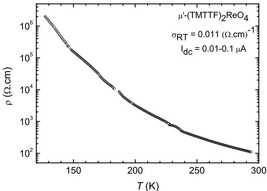
Figure 6.30. Resistivity measurements using the four-probe technique performed on a \mu' -(TMTTF) _2 ReO _4 thin single crystal. Reprinted with permission from Perruchas et al. , 2005.
