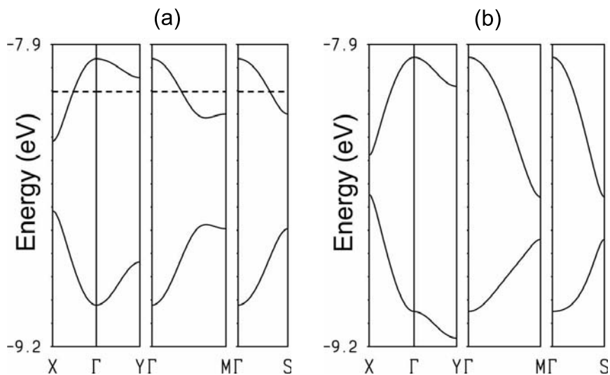
Figure 6.29. (a) Band structure of \mu' -(TMTTF) 2 ReO 4 . \Gamma = (0, 0) , X = (a^*/2, 0) , Y = (0, b^*/2) , M = (a^*/2, b^*/2) , S = (-a^*/2, b^*/2) with a' = \frac{1}{2}(b - a) and b' = \frac{1}{2}(a + b) . (b) Band structure of (TMTTF) 2 ReO 4 . Reprinted with permission from Perruchas et al. , 2005.
