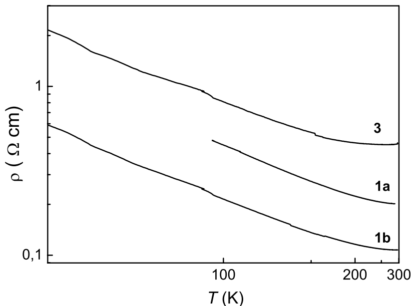
Figure 6.35. \rho(T) curves of thin TTF-TCNQ films grown at ( 1a and 1b ) T_{\text{sub}} = \text{RT} and T_{\text{ann}} \approx 350 \text{ K} and ( 3 ) T_{\text{sub}} \approx 325 \text{ K} and T_{\text{ann}} \approx 350 \text{ K} . The measurements were performed using the four contacts low-frequency lock-in technique with 10 \mu\text{A} for 1a and 0.1 \mu\text{A} for 1b and 3 . Reprinted from Journal of Solid State Chemistry , Vol. 168, J. Fraxedas, S. Molas, A. Figueras, I. Jiménez, R. Gago, P. Auban-Senzier and M. Goffman, Thin films of molecular metals: TTF-TCNQ , 384-389, Copyright (2002), with permission from Elsevier.
