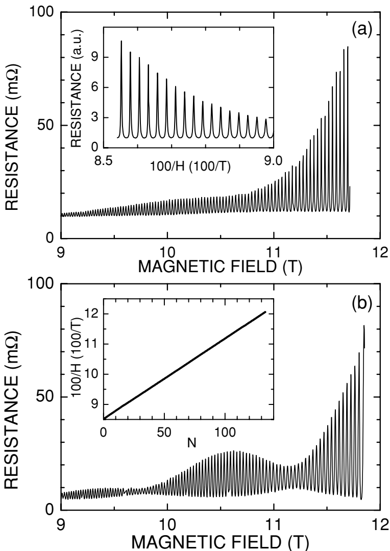
Figure 1.36. Magnetoresistance measurements performed between 9 and 12 T at 380 mK on two high-quality \beta_{\text{H}} -(BEDT-TTF) _2 I _3 single crystals (a) and (b). In the inset in (a) the high-field magnetoresistance at 380 mK is shown on an enlarged scale versus H^{-1} ( H represents \mathbf{B} ) and clearly reveals an enhanced anharmonicity at increased fields. The inset in (b) shows the inverse field values of 133 oscillation peaks vs. integral numbers. The almost perfect linearity is a test for both the origin of the oscillations and the quality of the data. The slope provides a fundamental field of 3730 T. Reprinted with permission from W. Kang, G. Montambaux, J. R. Cooper, D. Jérôme, P. Batail and C. Lenoir, Physical Review Letters , 62 , 2259 (1989). Copyright (1989) by the American Physical Society.
