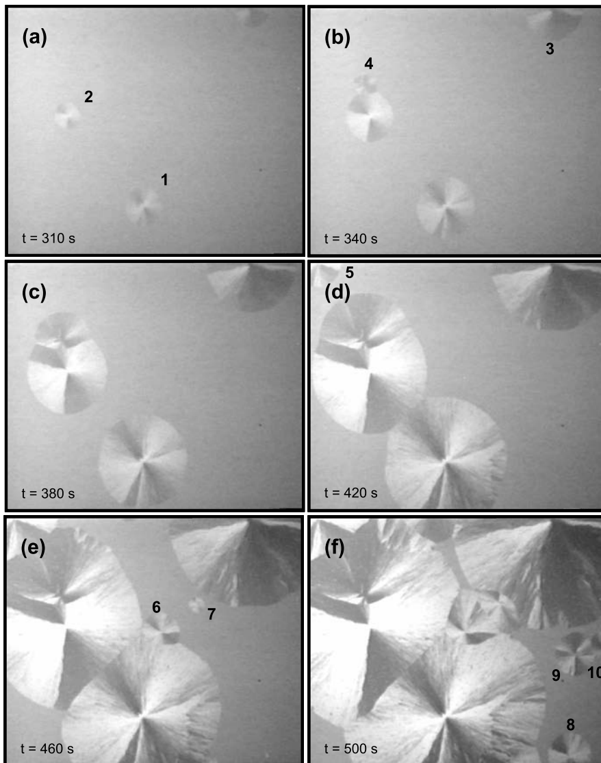
Figure 5.8. Time evolution of the 2D spherulitic crystallization of a thin film of p -NPNN during evaporation. In each picture ( 2.65 \times 2.20 \text{ mm}^2 , polarizers not completely crossed in order to avoid excessive loss of light) the deposition time is indicated. The 2D spherulites discussed in the text are labelled by order of formation. Reprinted from Journal of Crystal Growth , Vol. 209, J. Caro, J. Fraxedas and A. Figueras, Thickness-dependent spherulitic growth observed in thin films of the molecular organic radical p-nitrophenyl nitronyl nitroxide , 146–158, Copyright (2000), with permission from Elsevier. Details on the determination of the origin of the time scale ( t = 0 ) can be found in the original article.
