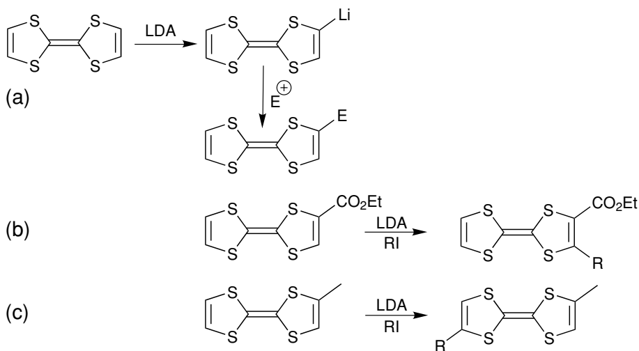
Figure 2.9. Electrophilic substitution of lithiated TTF (strategy S8). E stands for electrophilic substituent. (a) Generic reaction, (b) monosubstituted TTF with the electron withdrawing substituent CO_2Et and (c) monosubstituted TTF with the electron donor substituent CH_3 . E = Br, I, CO_2H, CO_2Et, CH_2OH, CH_3, CONR_2, CHNR_2, CHO , etc.
