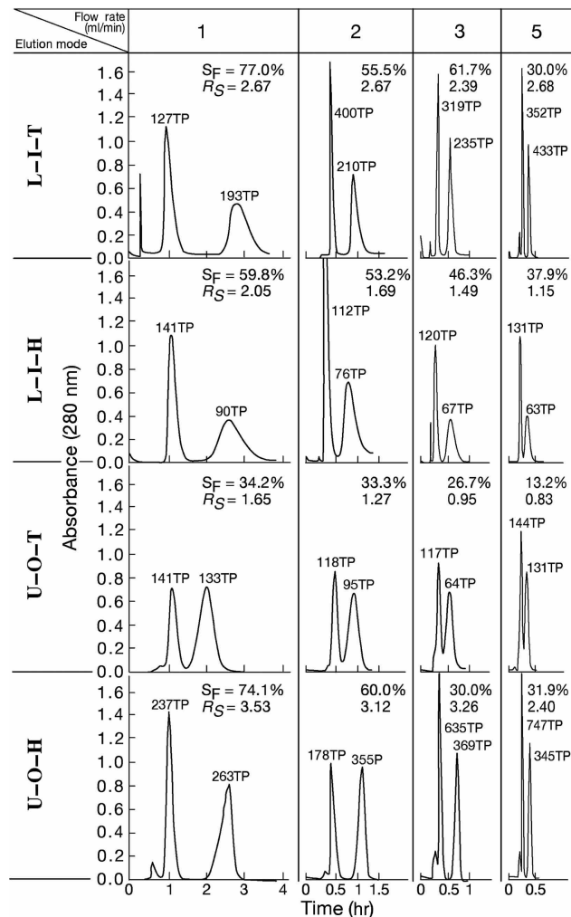
Fig. 12 Separation of dipeptides by spiral tube assembly at 800 rpm. Experimental conditions are as follows: apparatus: spiral tube with 1.6 mm I.D. and about 36 m long forming nine spiral layers with a total capacity of about 100 ml; solvent system: 1-butanol-acetic acid-water (4:1:5, v/v/v); Sample: trp-tyr (1.25 mg) and val-tyr (5 mg) in 0.5 ml of upper phase; monitoring system: Uvicord IIS at 280 nm; elution mode: L-I-T, lower phase pumped from the inner tail terminal of the spiral tube, L-I-H, lower phase pumped from the inner head terminal of the spiral tube, U-O-T, upper phase pumped from the outer tail terminal of the spiral tube, U-O-H, upper phase pumped from the outer head terminal of the spiral tube.
