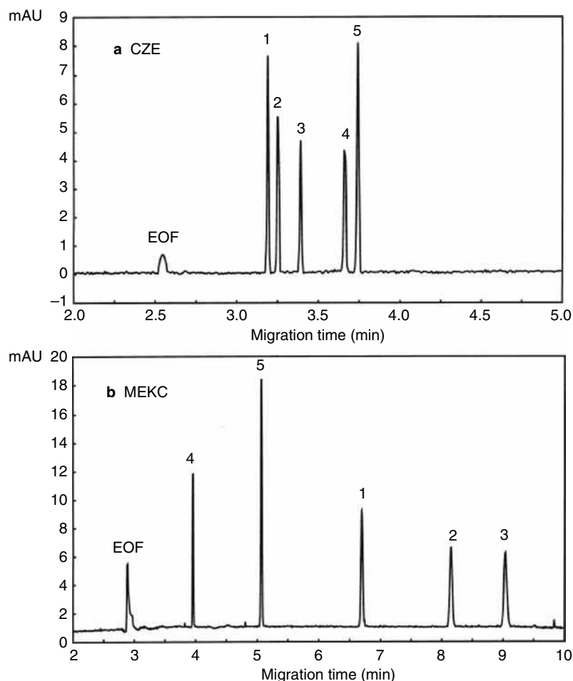
Fig. 2 Electropherograms of the separation of five barbiturate standards using a, CZE and b, MEKC. Peaks: 1, hexobarbital; 2, methohexital; 3, secobarbital; 4, barbital; and 5, phenobarbital.
