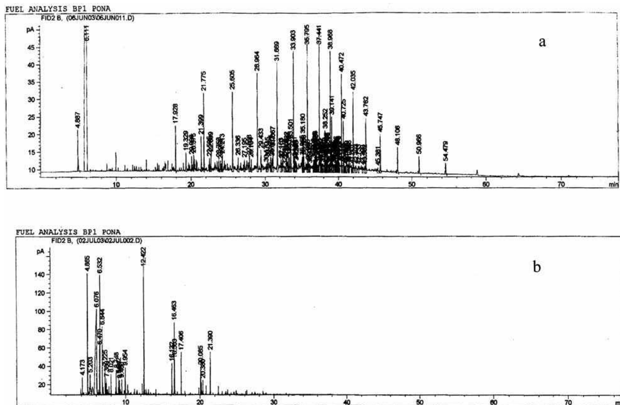
Fig. 2 GCs obtained after injecting 1 \mu l of (a) diesel and (b) unleaded gasoline. GC HP-6890 with FID, column BP1-PONA from SGE (50 m \times 0.15 mm \times 0.45 \mu m), injector temperature = 250°C, detector temperature = 300°C, oven temperature program = initial temp 40°C, rate 5°C/min, final temp 275°C. Carrier gas He with flow rate = 1 ml/min.
