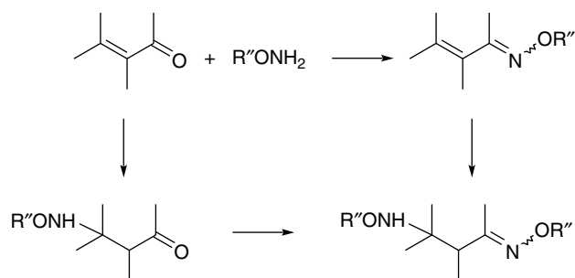
Fig. 3 Anomalous interaction of \alpha,\beta -unsaturated carbonyl compounds with O -alkyl hydroxylamines.
