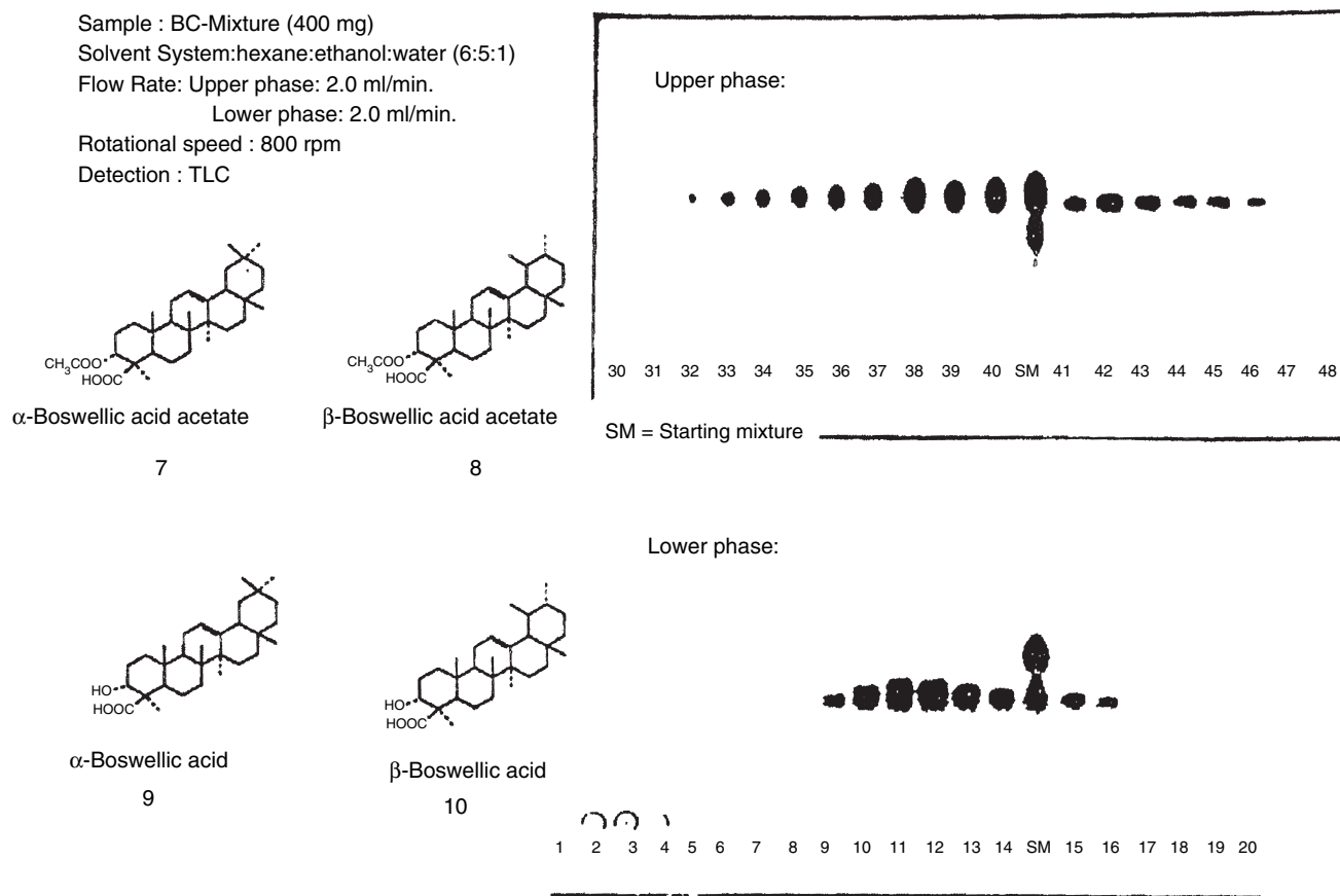
Fig. 2 DuCCC of triterpenic acids.
