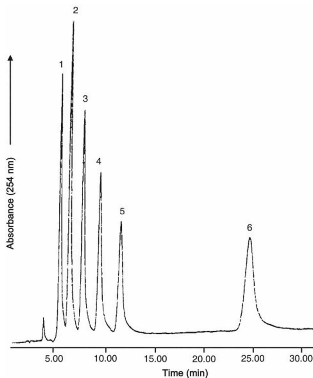
Fig. 1 Separation of RP test mixture on a C_{22} bonded phase. Mobile phase: 50 : 50 acetonitrile–water. Solutes: 1 = benzene; 2 = toluene; 3 = ethylbenzene; 4 = isopropylbenzene; 5 = t -butylbenzene; 6 = anthracene.
