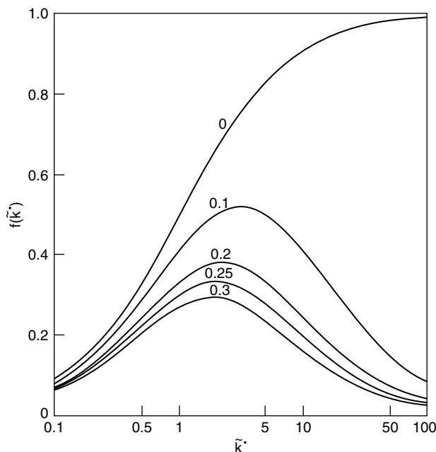
Fig. 1 Dependence of f(k) on capacity factor k . The values of \alpha are given on each line.
