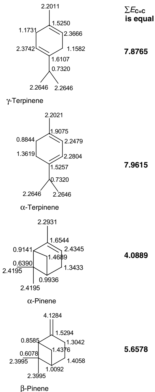
Fig. 1 The E-state values calculated for atoms of terpenes investigated and sum of electrotopological states ( \sum E_{C=C} ) for all carbon atoms forming double bonds.
