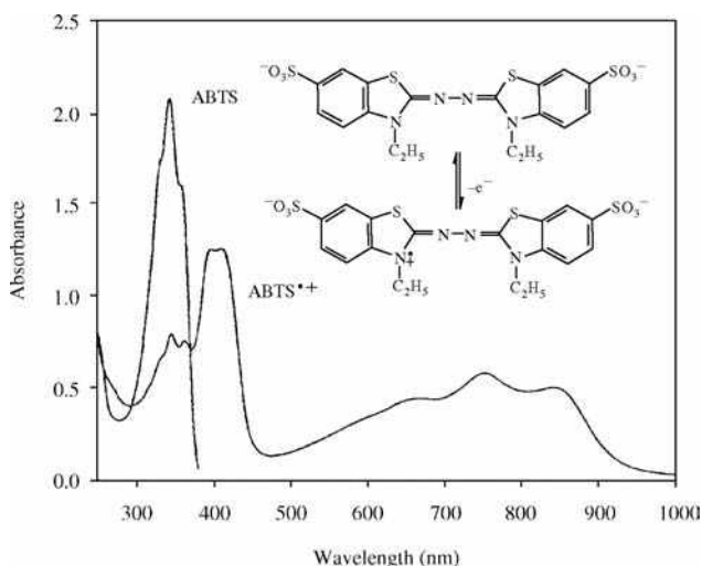
Fig. 1 Spectral characteristics of ABTS and its oxidation products, the ABTS radical (ABTS + ), showing absorbance of up to 1000 nm. The chemical structures show the nitrogen-centered radical cation of ABTS + .
