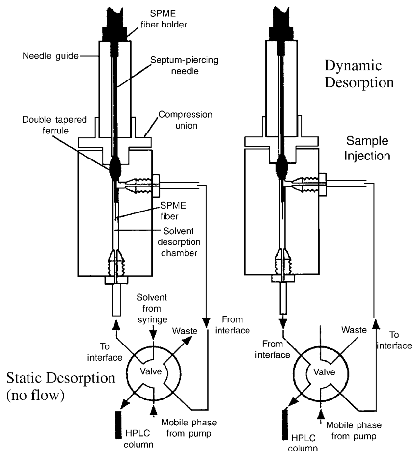
Fig. 6 SPME/HPLC interface.
