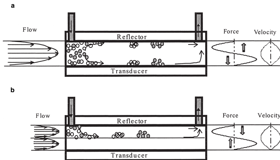
Fig. 1 Acoustic FFF channels suitable for particles with (a) A > 0 and (b) A < 0 , utilizing a divided acoustic FFF channel.
