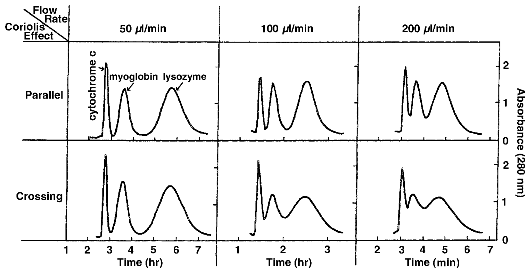
Fig. 2 Effects of Coriolis force on partition efficiency and retention of stationary phase in protein separation by toroidal coil centrifuge.
