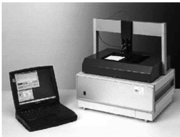
Fig. 4 J&M 2010 TLC Diode Array Scanner (TIDAS TLC 2010). Source: Photo courtesy of SpectrAlliance, Inc., St. Louis, Missouri.
