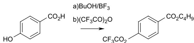
Fig. 2 Two-step derivatization of hydroxyarene-carboxylic acids.
