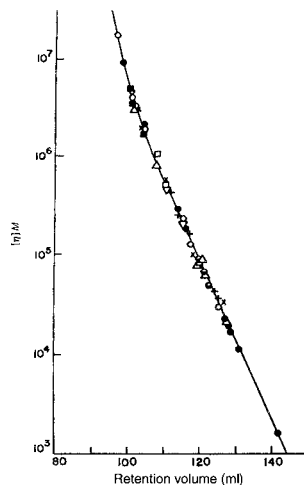
Fig. 1 Retention volume vs. [\eta]M .
