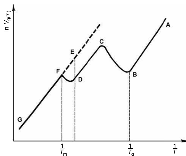
Fig. 3 The variation of the \ln V_{g(T)} vs. \frac{1}{T} for a semicrystalline polymer.
