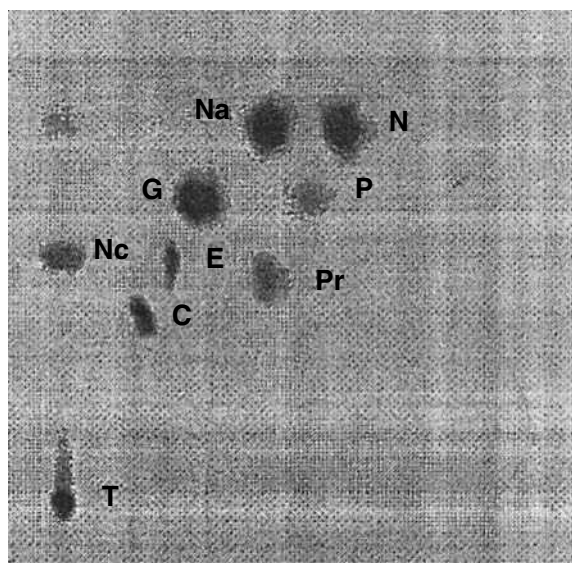
Fig. 2 Densitogram and videoscanned 2D-TLC of isoquinoline alkaloids separated on silica layer by use of aqueous methanol (8%) with 1% ammonia as the first direction eluent and multicomponent non-aqueous eluent with 0.1 M DEA as the second direction eluent. N—noscapine, Na—narcotine, Nc—narceine, G—glaucine, E—emetine, C—codeine, P—papaverine, Pr—protopine, T—tubocurarine. Source: From the effect of chromatographic conditions on the separation of selected alkaloids on silica layers, in J. Planar Chromatogr. [16]
