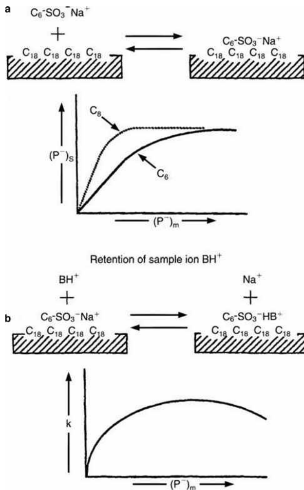
Fig. 2 Effect of ion-pair reagent concentration on separation. (a) Sorption of the ion-pair reagent as a function of concentration for reagents of different hydrophobicity ( \text{C}_6 - and \text{C}_8 -sulfonates); (b) retention as a function of reagent concentration.
