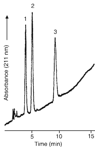
Fig. 2 Gradient separation of peptide mixture on a C_{30} bonded phase. Mobile phase, linear gradient from 25% to 45% A in 15 min. A = 0.1% trifluoroacetic acid (TFA) in 75 : 25 acetonitrile–water and B = 0.1% TFA in water. Solutes: 1 = bradykinin; 2 TFA angiotensin III; 3 = angiotensin I.
