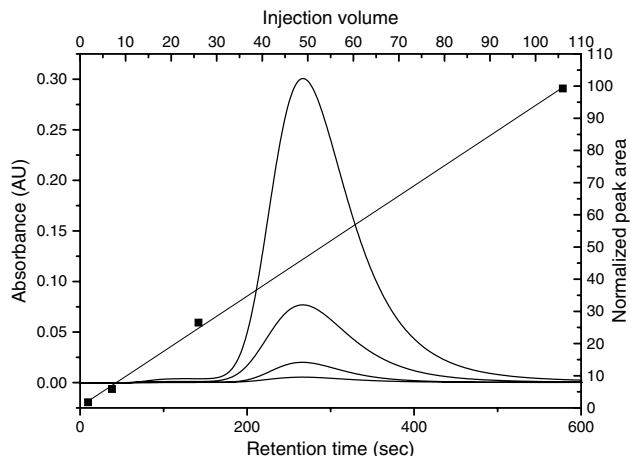
Fig. 2 Results showing pre-concentration of 1.7–106 ml of a natural freshwater sample using the procedure in Fig. 1. The solid lines show the UV detector response while the squares with regression line (slope 0.94 and R^2 0.9993) represent peak area vs. injection volume. The samples were first diluted in order not to exceed the overloading point. Source: From Optimisation of on-channel pre-concentration in flow field-flow fractionation for the determination of size distributions of low molecular weight colloidal material in natural waters, in Anal. Chim. Acta. [7]
