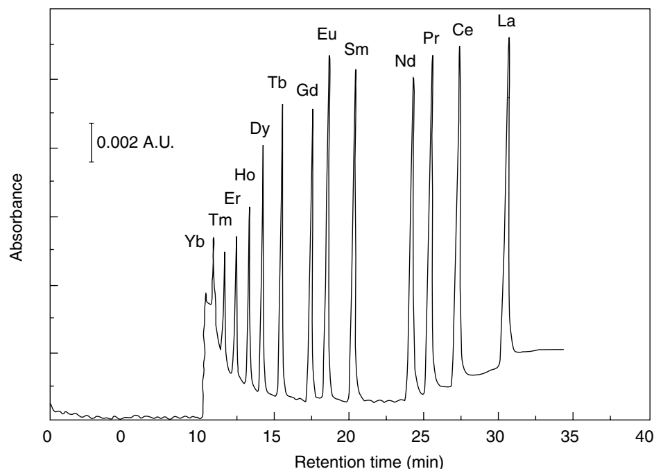
Fig. 4 Separation of lanthanides by HPLC. Experimental conditions: reversed phase column, 4.6 \times 150 mm 5 \mu\text{m} Supelcosil LC-18 coated with 2.5 \times 10^{-4} M C_{20}SO_4^- in 25% acetonitrile-water; eluent, 0.025 M \alpha -HIBA (pH 3.8) for 9 min followed by linear gradient from 0.025 to 0.25 M \alpha -HIBA (pH 3.8) over 20 min; detection, 658 nm after postcolumn reaction with Arsenazo III.
