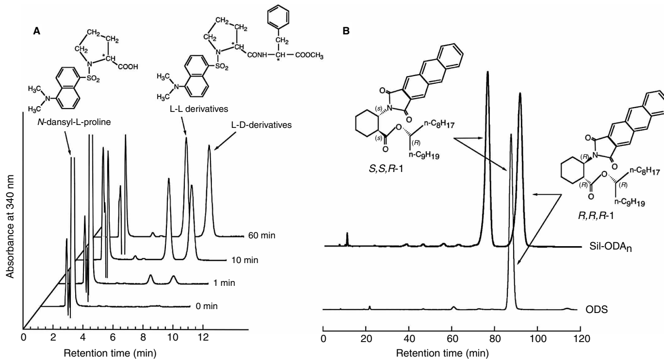
Fig. 10 (A) Time course of diastereomerization of dl-phenylalanine with N -dansyl-L-proline using DEPC [24] and (B) chromatograms of the mixture of S,S,R-1 and R,R,R-1 with Sil-ODA n and ODS. [25] Mobile phases: (A), methanol–water (7:3) at 25°C; (B), methanol at 0°C.
