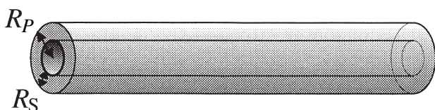
Fig. 1 The volume accessible to the center of a spherical molecule of radius R_s within a cylindrical pore of radius R_p is the interior cylinder of radius R_p - R_s .
