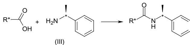
Fig. 6 An example of the formation of diastereomeric amides from chiral carboxylic acids and ( S )- \alpha -methylbenzenemethanamine.
