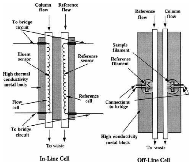
Fig. 1 Katharometer cells.
