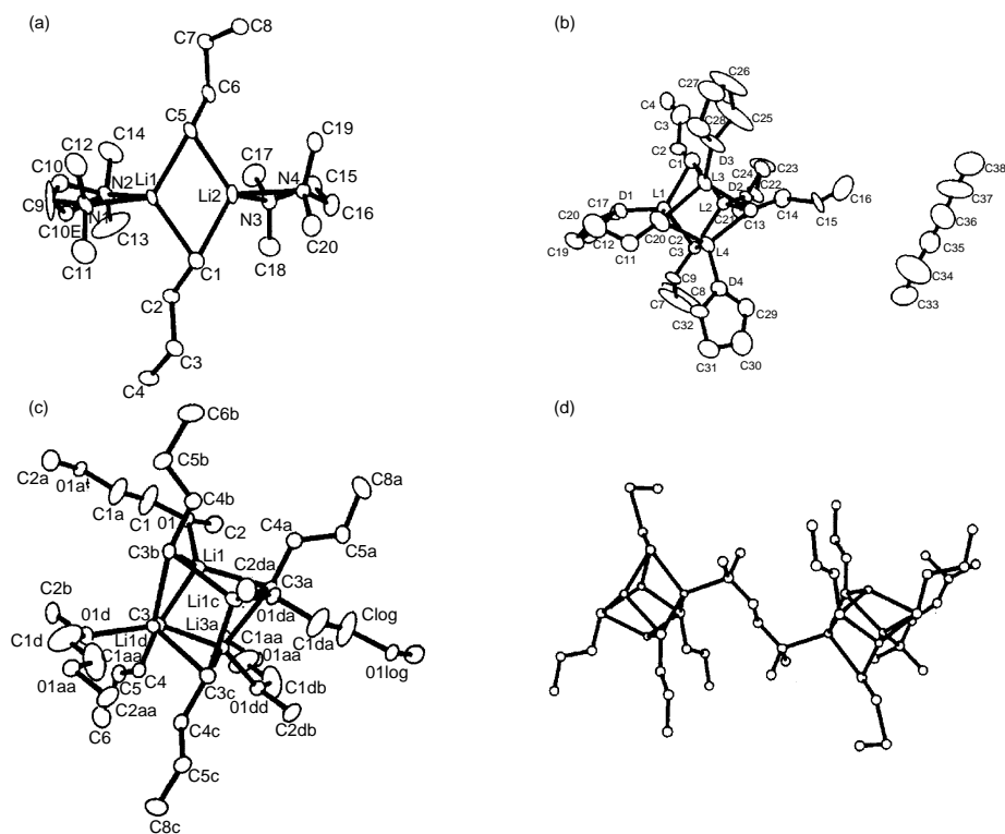
Fig. 6.2. Crystal structures of n -butyllithium: (a) [(n\text{-BuLi-TMEDA})_2]_2 ; (b) [(n\text{-BuLi-THF})_4]\text{hexane} ; (c) [(n\text{-BuLi-DME})_4] ; (d) [(n\text{-BuLi})_4]\cdot\text{TMEDA} . Reproduced from J. Am. Chem. Soc. , 115 , 1568, 1573 (1993), by permission of the American Chemical Society.
