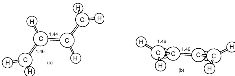
Fig. 12.26. Computed initial excited state structures of butadiene. (a) s-trans S_1 ; (b) s-cis S_1 . Reproduced from J. Am. Chem. Soc. , 115 , 3710 (1993), by permission of the American Chemical Society.
