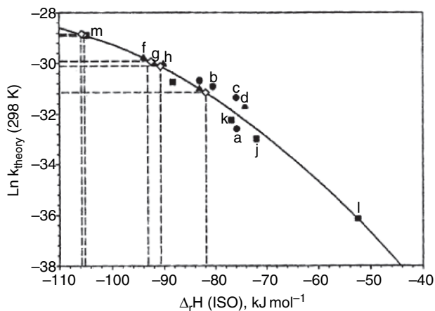
Fig. 11.20. Quadratic Evans-Polanyi relationship \ln k(298) = -1.368 \times 10^{-3} \Delta H_f^2 - 0.354 \Delta H_f - 50.96 : (a) CH 3 F, (b) CH 3 Cl, (c) CH 3 Br, (d) CH 2 F 2 , (e) CH 2 FCl, (f) CH 2 Cl 2 , (g) CH 2 ClBr, (h) CH 2 Br 2 , (i) CHF 3 , (j) CHF 2 Cl, (k) CHF 2 Br, (l) CHFCl 2 , (m) CHCl 3 . From J. Phys. Chem. A , 105 , 1599 (2001).
