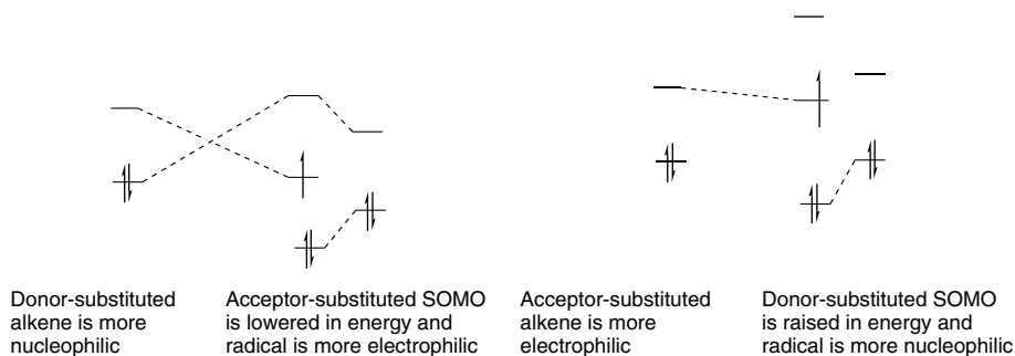
Fig. 11.6. Frontier orbital interactions between different combinations of substituted radicals and alkenes showing enhanced interaction relative to unsubstituted systems.
