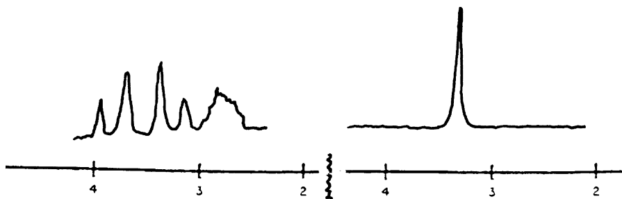
Fig. 2.16Pa. Partial ^1\text{H} NMR spectra of cis and trans isomers of 1-benzyl-2,6-dimethylpiperidine. Reproduced by permission of Elsevier.
