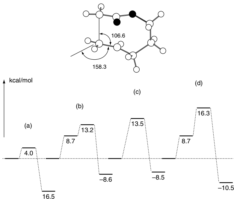
Fig. 11.10. Comparison of energies of (a) 8-endo-s-cis, (b) 8-endo-s-trans, (c) 7-exo-s-cis, and (d) 7-exo-s-trans transition structures. Reproduced from J. Am. Chem. Soc. , 120 , 7469 (1998), by permission of the American Chemical Society.
