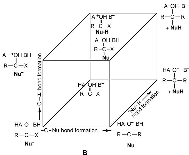
Fig. 3.6. Reaction progress cube showing possible intermediates for nucleophilic addition to a carbonyl group involving HA, \text{B}^- , and Nu-H. Adapted from J. Org. Chem. , 55 , 4238 (1990).
