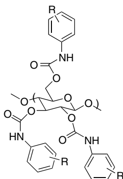
repeating unit for tris -carbamoyl derivatives of cellulose
