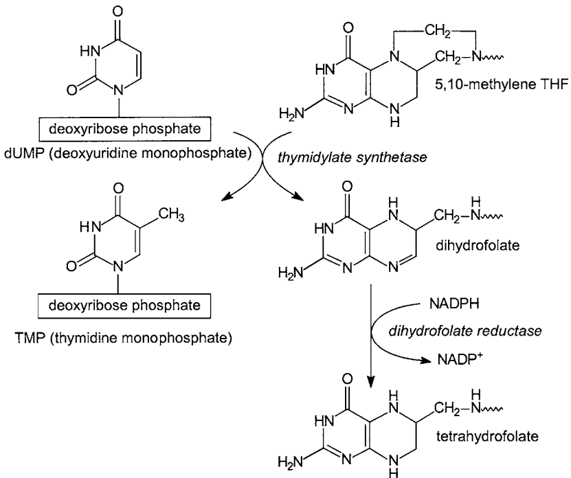
Figure 10.8. Synthesis of thymidine monophosphate. Thymidylate synthase, EC 2.1.1.45; and dihydrofolate reductase, EC 1.5.1.3. THF, tetrahydrofolate.
