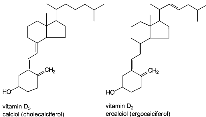
Figure 3.1. Vitamin D vitamers. Relative molecular masses ( M_r ): calcitol, 384.6; ercalcitol, 396.6.
