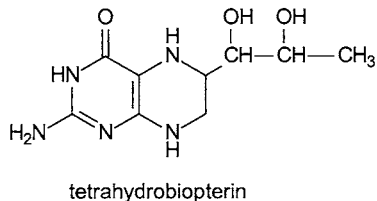
Figure 10.1. Folate vitamers, the folate antagonist methotrexate, molybdopterin, and tetrahydrobiopterin. Relative molecular masses ( M_r ): tetrahydrofolic acid, 445.4; methotrexate, 454.5; and tetrahydrobiopterin, 290.3.
