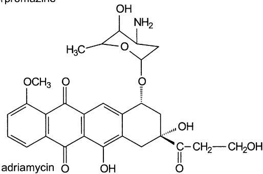
Figure 7.6. Drugs that are structural analogs of riboflavin and may cause deficiency. Relative molecular masses ( M_r ): riboflavin, 376.4; quinacrine, 472.9 (dihydrochloride); chlorpromazine, 318.9; imipramine, 280.4; amitriptyline, 277.4; and adriamycin (doxorubicin), 543.5.
