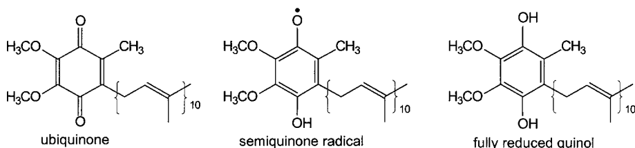
Figure 14.8. Ubiquinone. Relative molecular mass ( M_r ): 863.3.
