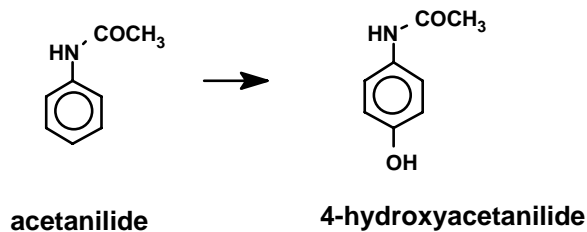
SCHEME 11.10 Acetanilide, like phenobarbital discussed previously, exemplifies the aromatic compounds that rearrange rapidly following CYP-mediated arene epoxide formation.
