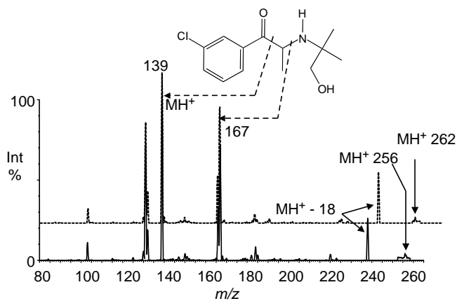
FIGURE 12.13 Collision-induced MS/MS spectra of the \text{MH}^+ ions at m/z 256 and 262 of hydroxybupropion (solid line) and [\text{2H}_6] hydroxybupropion (dotted line). Note that the fragment ions do not display the characteristic chlorine isotope pattern because only the higher abundance ^{35}\text{Cl} species was selected for MS/MS. The origin of fragments at m/z 167 and 139 is shown; neither retains deuterium atoms present in the internal standard. Data provided by R.L. Walsky and R.S. Obach, Pfizer, New York, NY.
