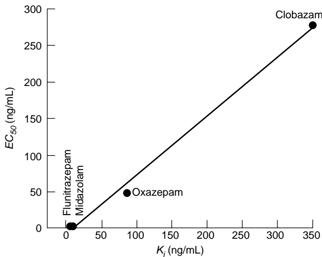
FIGURE 19.5 Relationship in rats between the EC_{50} of EEG effects (averaged amplitude in the 11.5–30 Hz frequency band) and estimates of K_i obtained from in vitro studies of the ability of four benzodiazepines to displace [3H]flumazenil from benzodiazepine receptors on brain tissue homogenates. Estimates of EC_{50} were based on free benzodiazepine concentrations not bound to plasma proteins. (Data from Mandema JW, Sansom LN, Dios-Vièitez MC, Hollander-Jansen M, Danhof M. J Pharmacol Exp Ther 1991;257:472–8.)
