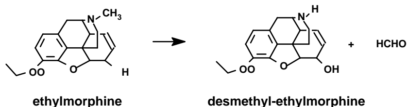
SCHEME 11.13 Ethylmorphine exemplifies drugs metabolized by N-dealkylation; other drugs similarly metabolized include lidocaine, aminopyrine, acetophenetidine, and 6-methylthiopurine.
