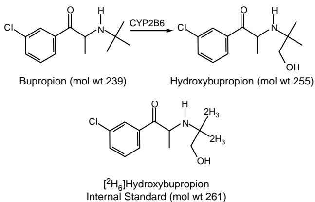
FIGURE 12.11 Metabolism of bupropion by CYP2B6 to hydroxybupropion and the structure of the stable isotope-labeled internal standard [ 2 H 6 ]hydroxybupropion.
