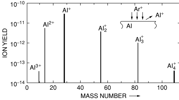
FIGURE 4.8. Secondary ion cluster spectrum from Ar + ion bombardment of Al. Note that the ordinate is a log scale. The predominant species is Al + , but Al 2 + and Al 3 + are also in abundance. [From Werner, 1978, with permission from Springer Science+Business Media.]
