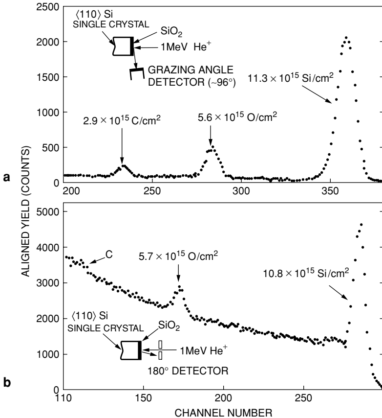
FIGURE 5.20. Energy spectra taken in channeling configuration from an Si(110) single crystal with a = 0.15 nm of SiO 2 . The top figure shows a detector placed at grazing exit angle geometry; the bottom figure shows a detector placed at \sim 180^\circ .
