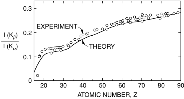
FIGURE 11.13. Measured K_\beta/K_\alpha ratios as a function of atomic number. The theoretical curve represents a more sophisticated treatment that includes all electronic wave functions. The hydrogenic atom model result for I(K_\beta)/I(K_\alpha) is 0.25. [From Bambynek et al., 1972, © 1972 by The American Physical Society.]
